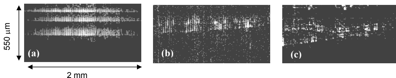
Figure 5. OCT results from above (a) a 200 \mu\text{m} thick microscope cover slip, and below a sample of spring onion showing (b) single-shot image with two visible layers, (c) an average of five images, displaying three visible layers, with translation of the raster between acquisitions.
