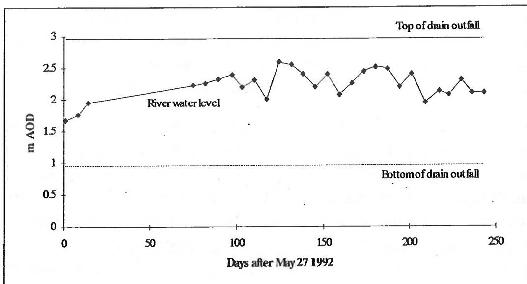
Figure 4: River Water Levels and Outfall Levels - Drain 38 (near Misson)
