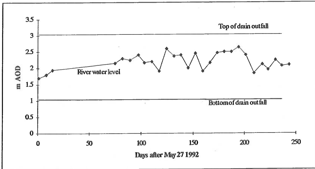
Figure 3: River Water Levels and Outfall Levels - Drain 38 (nr Idle Stop).
