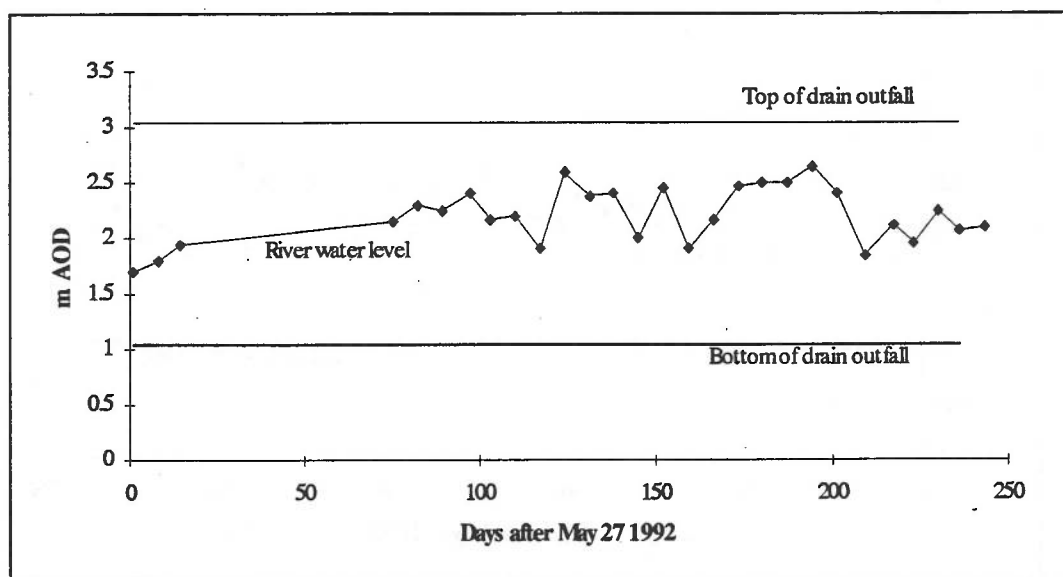
Figure 5: River Water Levels and Outfall Levels - Drain 35 (u/s of Misson)
