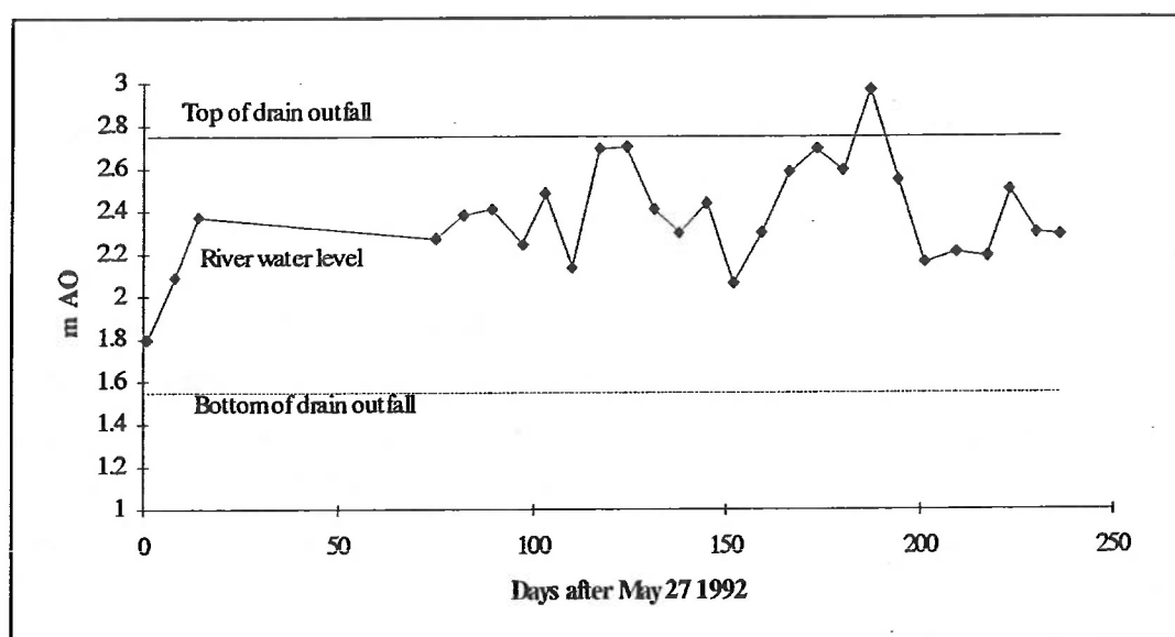
Figure 6: River Water Levels and Outfall Levels - Drains 44 & 49 (u/s Bawtry Bridge)
