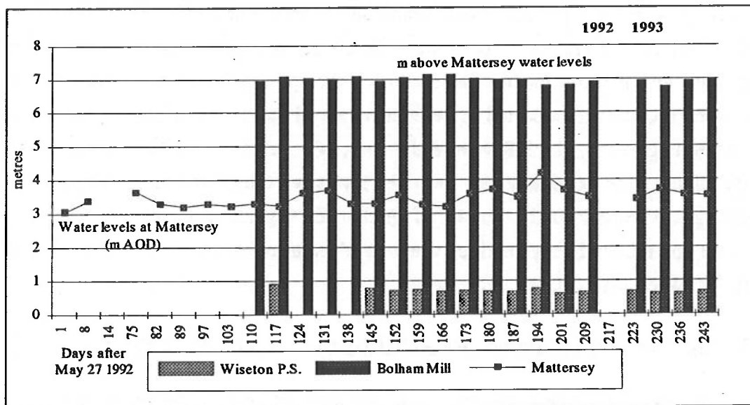
Figure 2: River Water Levels at Mattersey and Change in Levels at Wiseton Pumping Station and Bolham Mill relative to Mattersey
