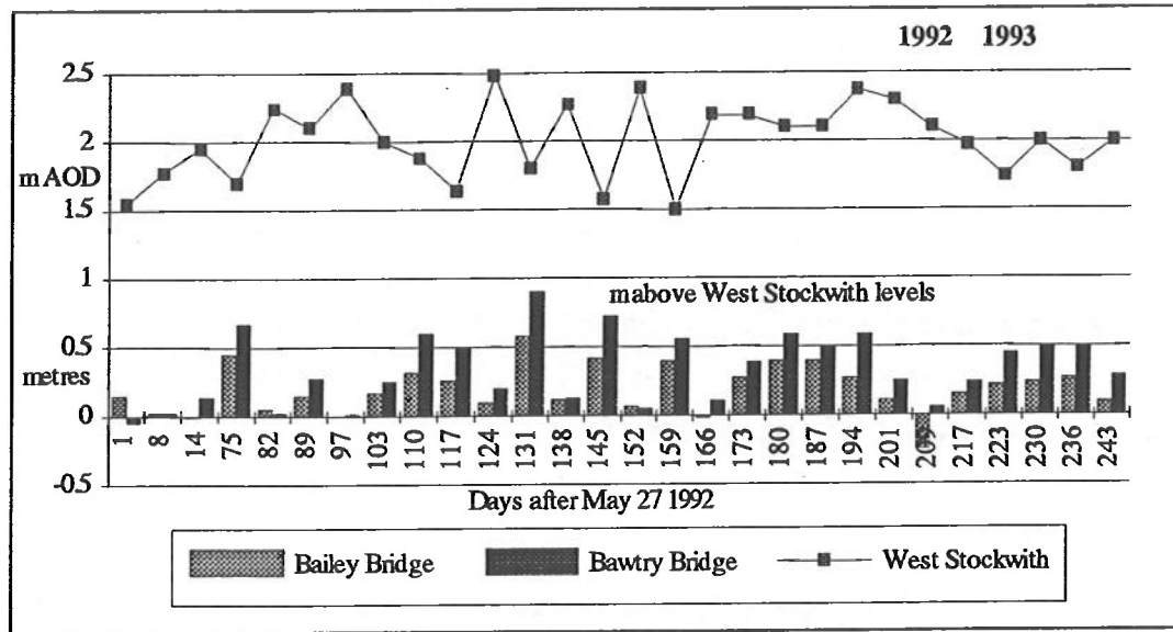
Figure 1: River Water Levels at West Stockwith and Change in Levels at Bailey Bridge and Bawtry Bridge relative to West Stockwith
