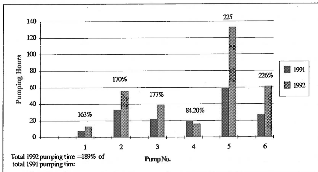
Figure 7: Pumping Times at Wiseton Pumping Station (1991/1992)
