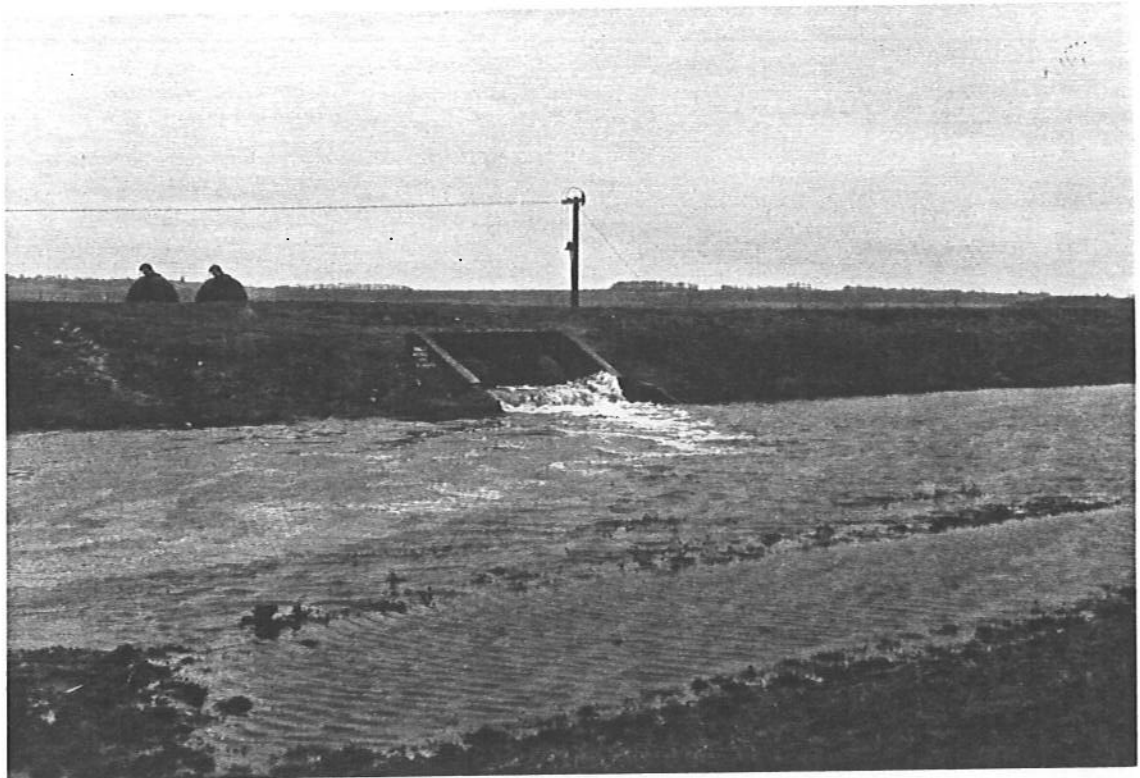
Plate 1: Gringley Pumping Station (Everton IDB) in action - July 1992
