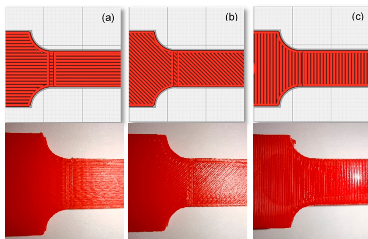
Figure 1. Building orientations directions and angles: (a) X (0°); (b) XY (±45°); and (c) Y (90°) [33].
