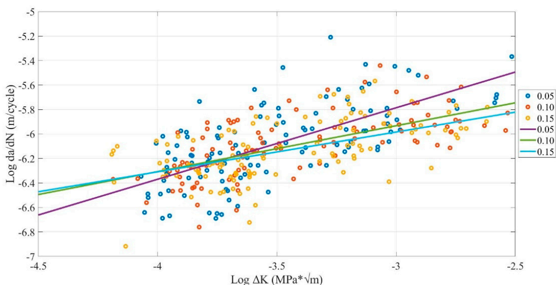
Figure 10. Comparison between layer thickness influence on FCG rate of FDM ABS samples with (0.4-, 0.6-, and 0.8-mm nozzle size, and X, XY, and Y building orientation) under 50, 60, 70 °C environmental temperatures.
