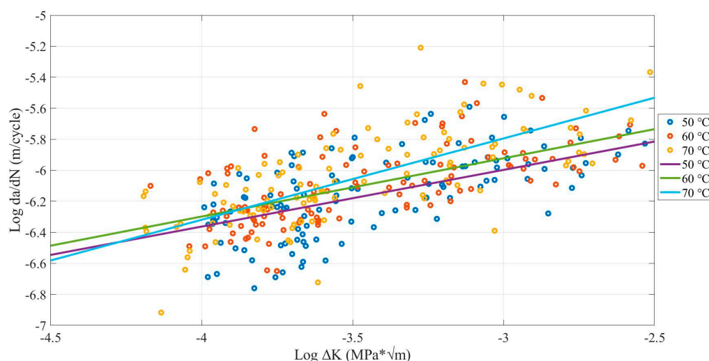
Figure 14. Comparison between the environmental temperatures influence on FCG rate of FDM ABS samples printed with (0.05-, 0.10-, and 0.15-mm layer thickness; 0.4-, 0.6-, and 0.8-mm nozzle sizes; and X, XY, and Y building orientations).
