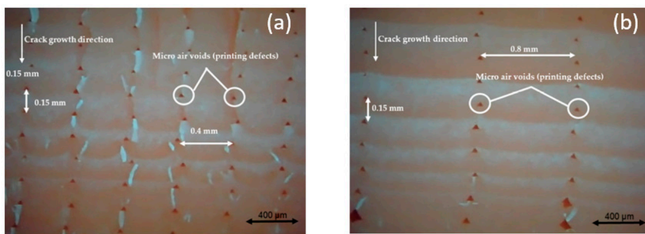
Figure 13. Comparison between the influence of different nozzle sizes of FDM ABS, printed with 0.15-mm layer thickness, X building orientation, and nozzle size (a) 0.4 mm and (b) 0.8 mm [33].
