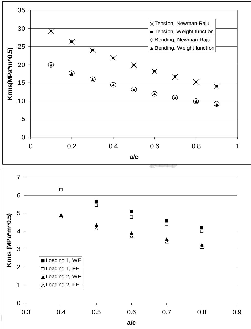
Fig. 4- Comparison between the weight function and the finite elements results for different loadings:
