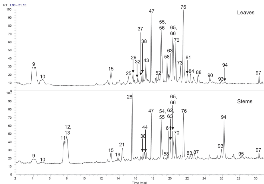
Figure 1. Total ion chromatograms (negative ion mode) of the leaves and stems of V. gummifera extracted with \text{H}_2\text{O}:\text{CH}_3\text{OH} (4:1 v/v).
