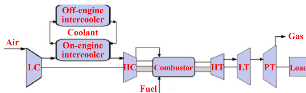
Figure 13. Intercooled-cycle gas turbine schematic diagram.
