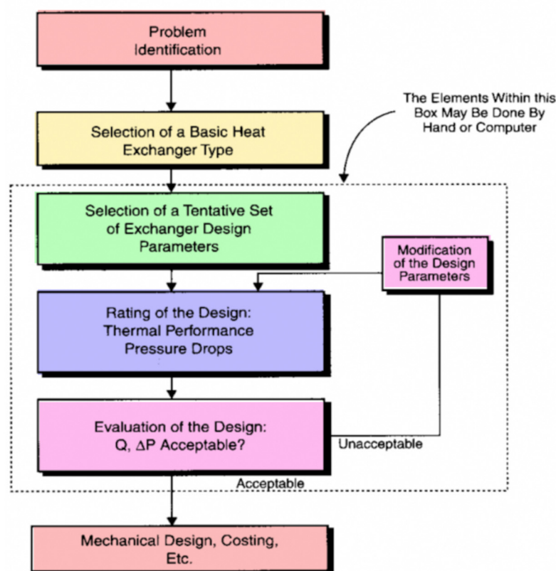
Figure 26. Shows a flow chart for the thermal design of HEs.
