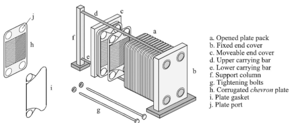
Figure 28. Typical structure of plate-fin heat exchanger with chevron plates [61].
