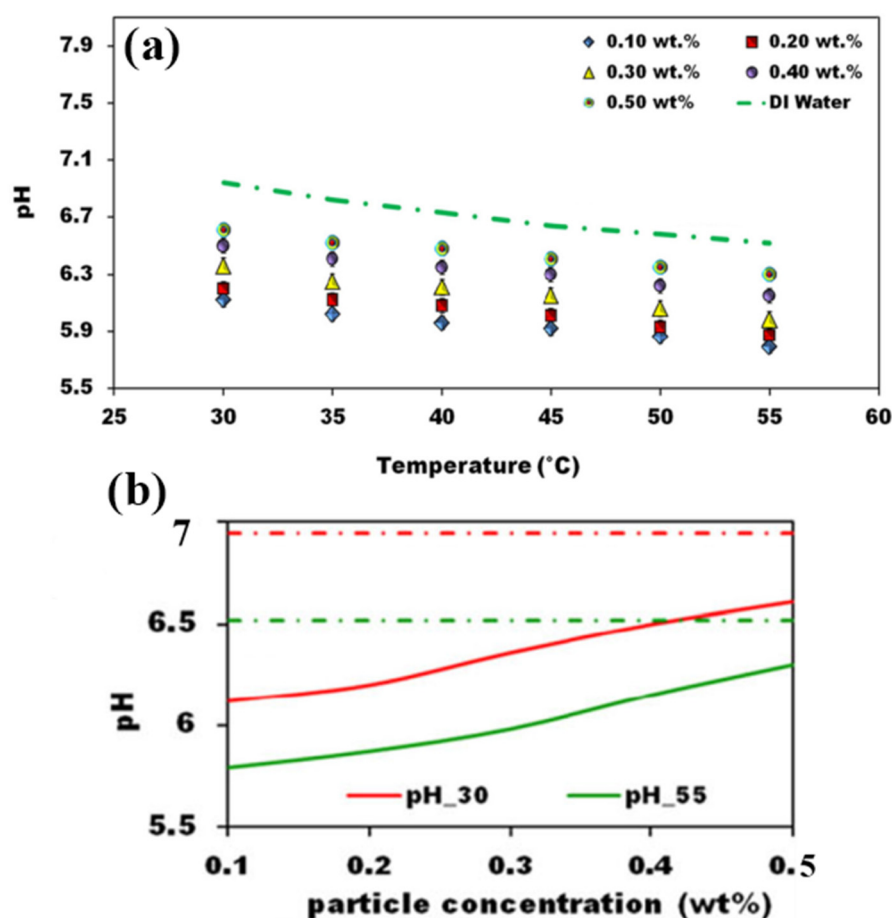
Figure 46. Changes in pH, where (a) shows the variation of the pH value of \text{Al}_2\text{O}_3 nanofluid at different nanoparticles concentrations, and (b) demonstrate the changes in the magnitude of the pH value at two different temperatures.
