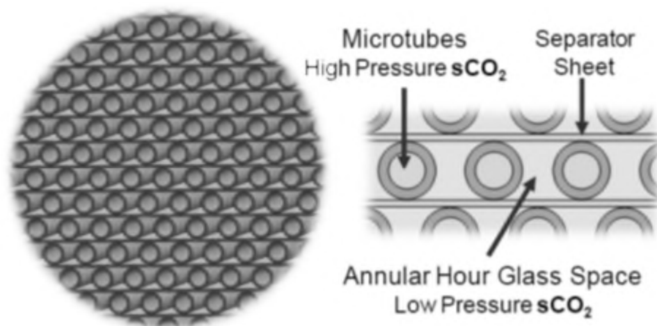
Figure 27. Recuperator tube bundle cross-section.
