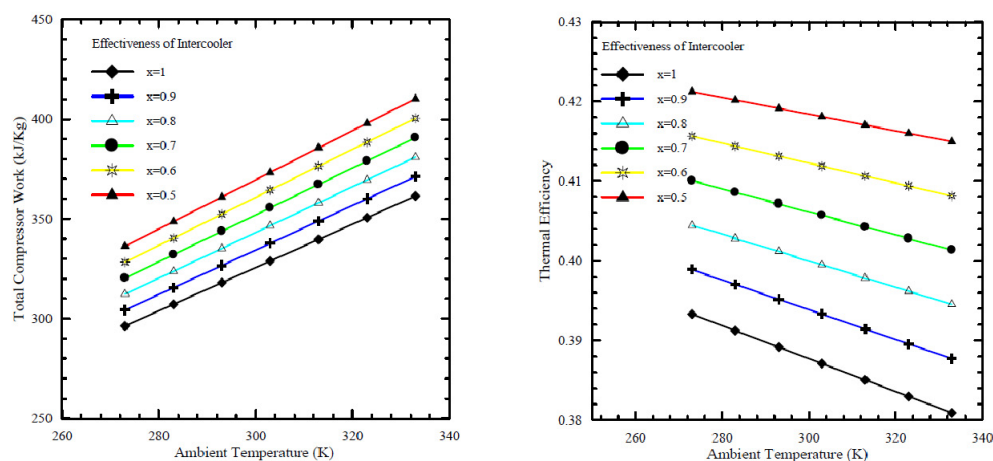
Figure 12. Effect of ambient air temperature to inlet compressor on the performance of Brayton cycle with different intercooler effectiveness [18].
