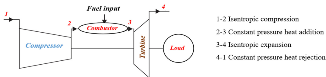
Figure 1. Schematic representation of a simple cycle gas turbine without intercooler [2].
