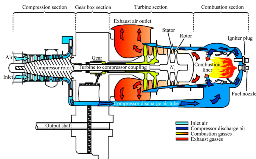
Figure 5. Turboshaft gas turbine engine instruction [11].
