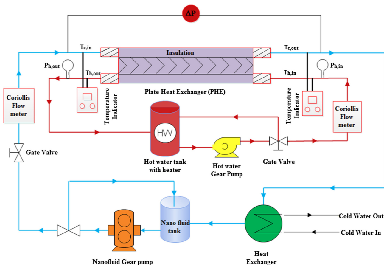
Figure 35. Schematic of experimental apparatus used by Kumar et al. [83].
