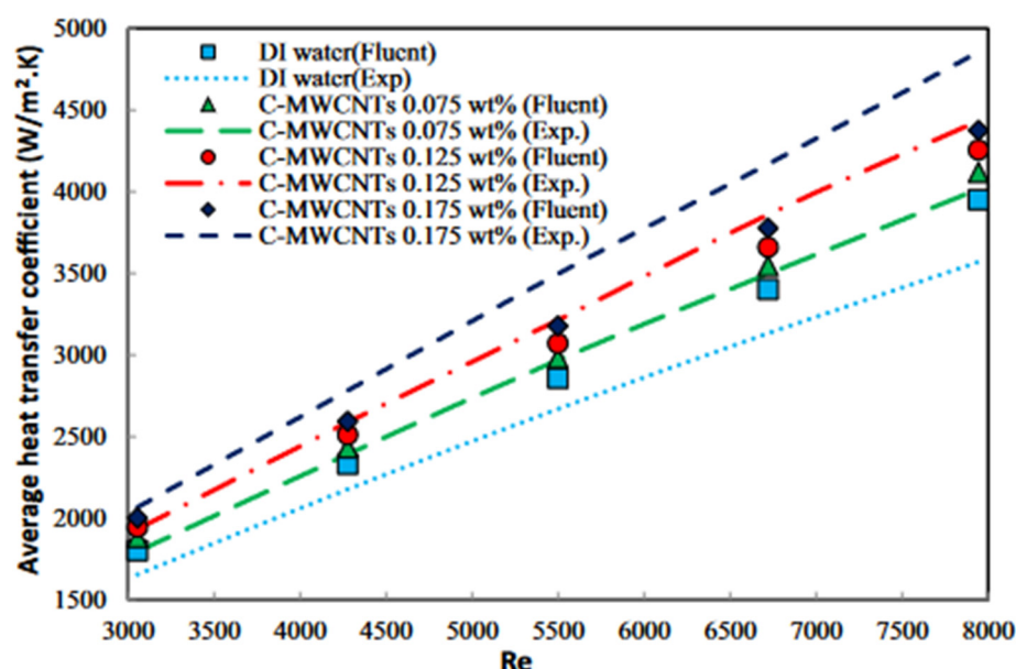
Figure 34. Variation of the average heat transfer coefficient with respect to the Reynolds number for C-MWCNT/distilled water nanofluids in a concentric annular heat exchanger.
