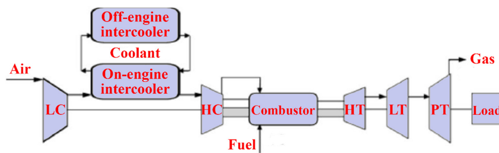
Figure 13. Intercooled-cycle gas turbine schematic diagram.
