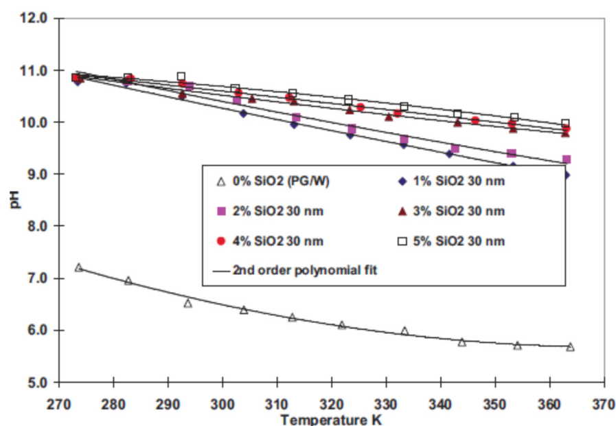
Figure 44. pH as a function of temperature for SiO 2 nanoparticles in PG/W (60:40) base fluid for particle concentration ranging from 0 to 5.0 vol.% [115].
