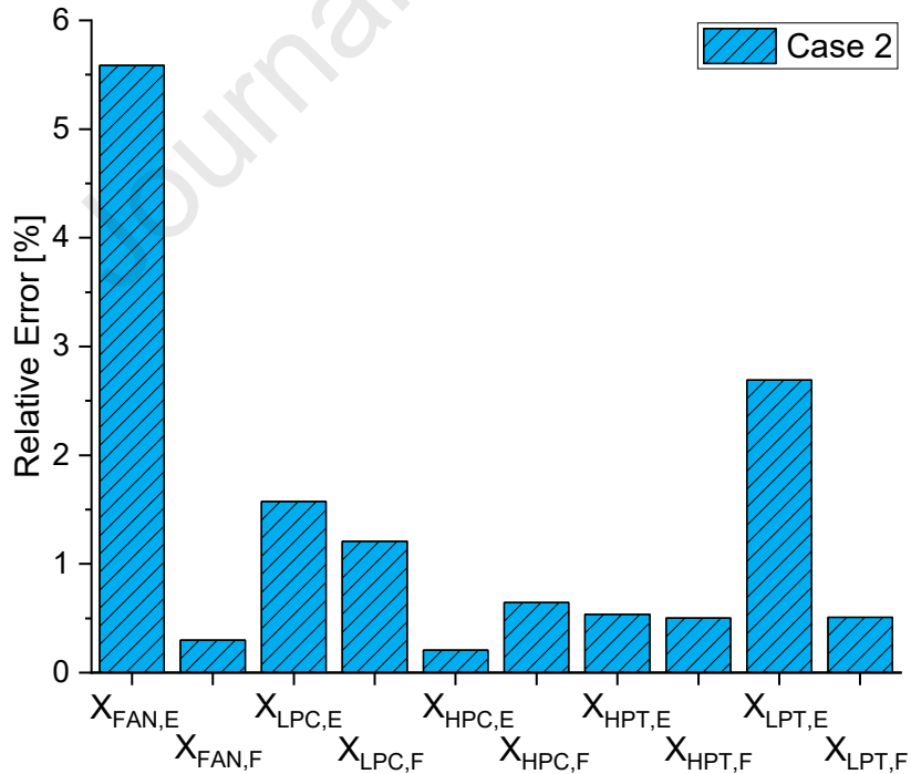
Fig. 11 Average relative error of health parameters during a transient maneuver.
