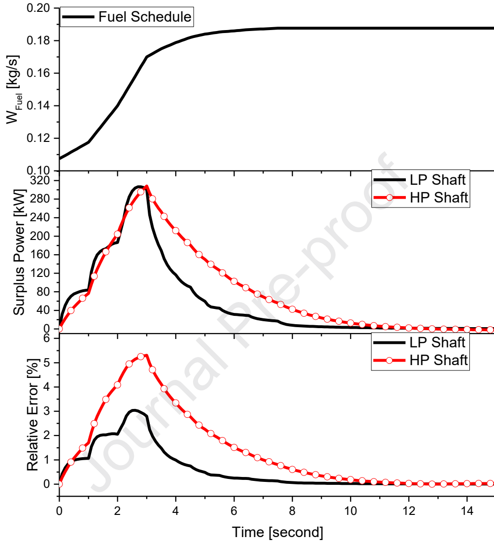
Fig. 6 Fuel schedule and power imbalance between CW and TW during a transient maneuver.
