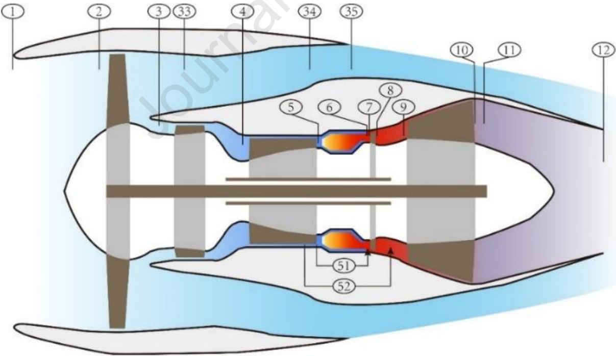
Fig. 2 Configuration of turbofan engine in concern and its station numbering [13].
