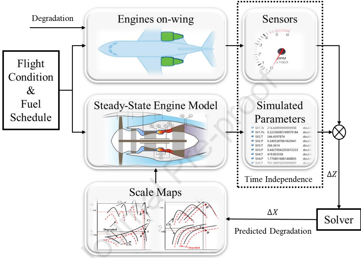
Fig. 3 Schematic of benchmark fault diagnosis method [13].
