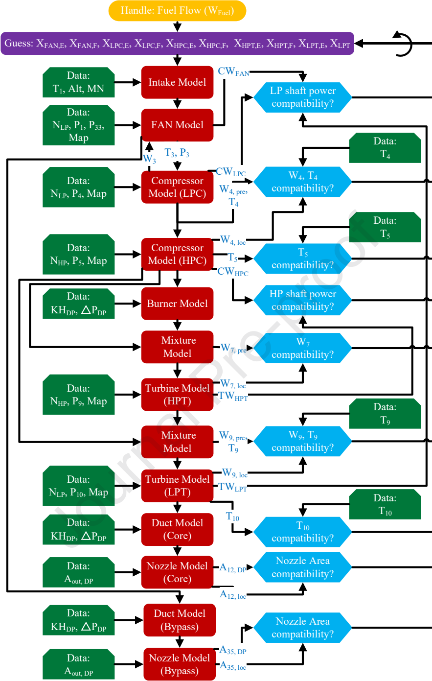
Fig. 4 Fault diagnosis based on steady-state model.
