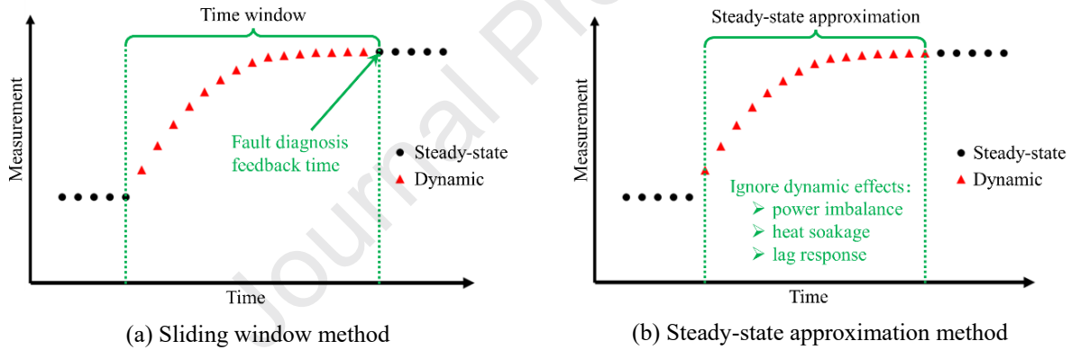
Fig. 1 Fault diagnosis methods at transient conditions.
