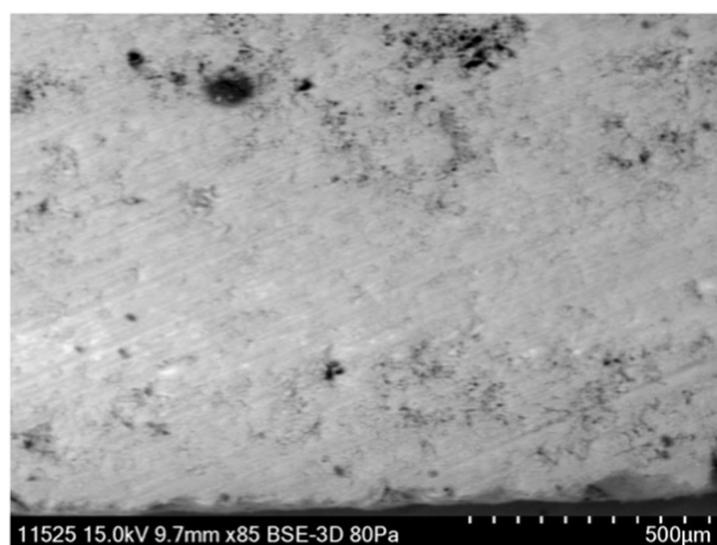
Fig. 5. Outer edge of bone 11,525, showing regions assumed to be associated with bacterial colonies.
