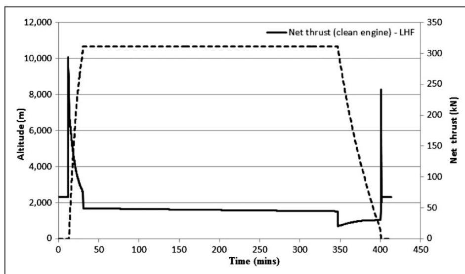
Figure 10. Change in altitude /mission profile and net thrust with time – LHM.
