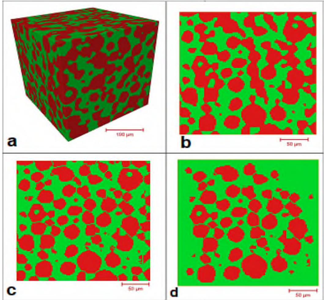
Figure 2 Image processing analysis to extract the pore size distribution in powder samples: (a) 3D reconstruction and color inversion of the pores and gaps, (b) 2D representation of a single slice, (c) isolating of the bonded particles, and (d) removal of the margins.
