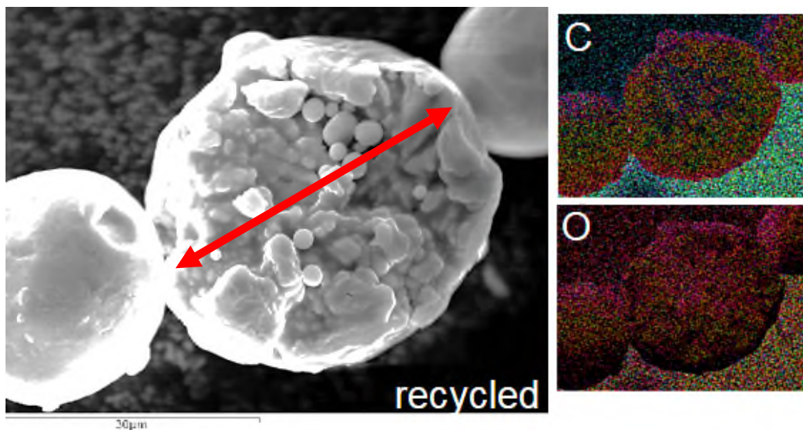
Figure 5 Open pore in a recycled particle images with EDX. The carbon and oxygen composition map across the pore shows a uniform distribution of the two elements. The red arrow shows the EDX line scan direction.
