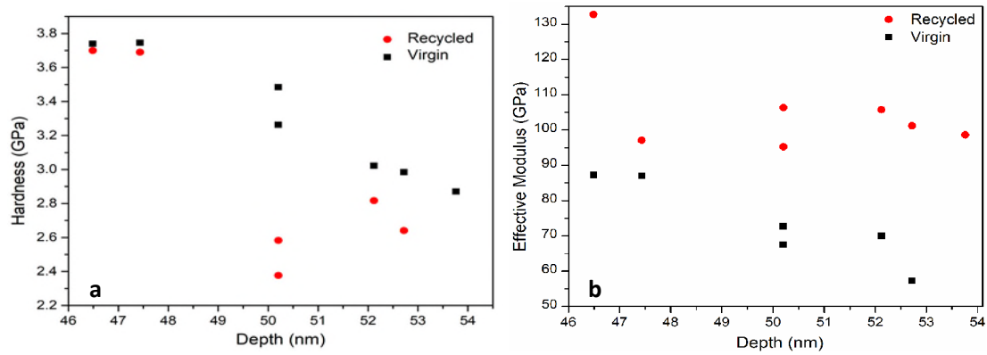
Figure 8 Nanoindentation measurements showing the (a) hardness and (b) effective modulus obtained for both recycled and virgin powder on different indentation on different porous locations of the particles.
