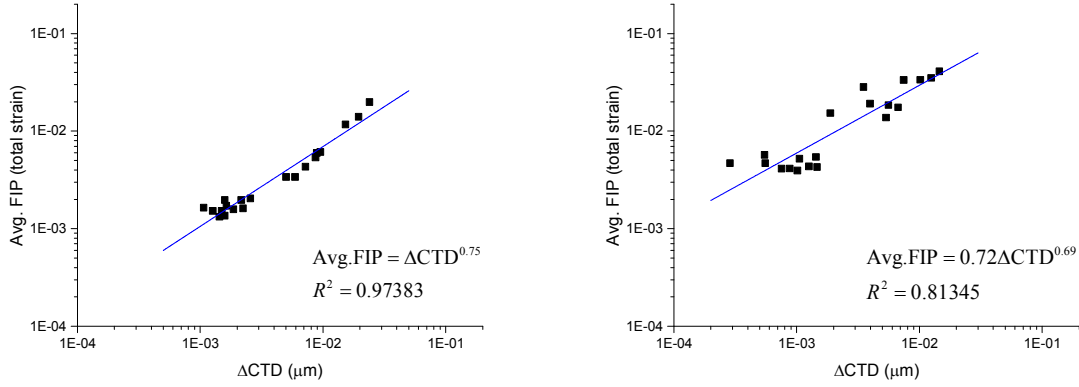
Figure 6. Comparison of computed SB-averaged FIP vs. \Delta\text{CTD} for (left) shear and (right) mixed mode loading.
