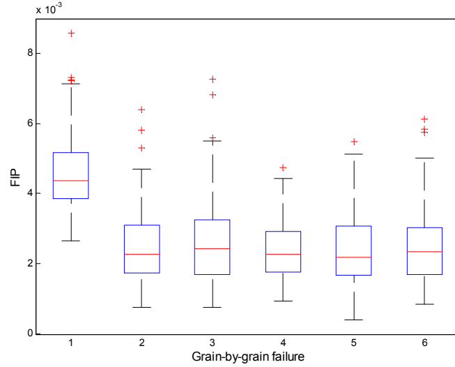
Figure 8. Distribution of maximum FIPs for the first six grains that failed from among all 150 simulations.
