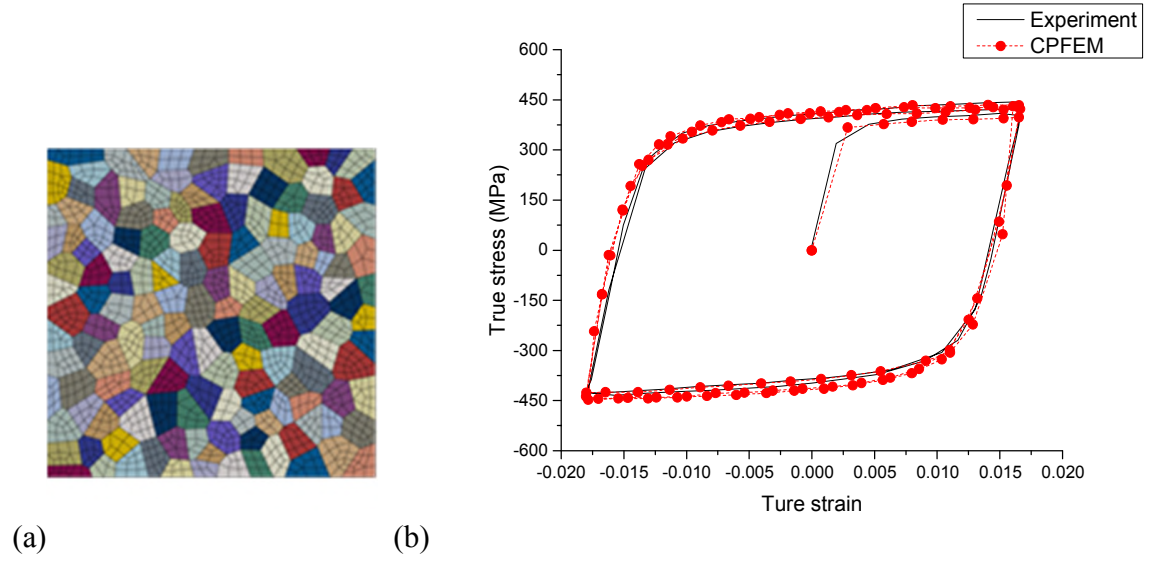
Figure 3. (a) FE mesh for a 400\ \mu\text{m} \times 400\ \mu\text{m} model with 150 grains, 1386 CPE4 elements, and fully periodic boundary condition (b) Stress–strain response from simulations and experiments ([52]). Note that the constitutive behavior from simulations saturates rapidly and the stress-strain loop after two computational cycles matches the saturated experimental curve.
