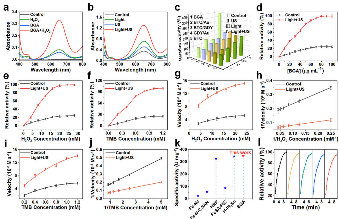
Fig. 2 (a), (b) and (c) Comparison of POD-like activities among various nanozymes. The reaction conditions were 25 °C for 10 min in buffer (pH 4.0). (d), (e) and (f) Comparison of POD-like activities of BGA at various concentration (0–100 \mu\text{g mL}^{-1} ), \text{H}_2\text{O}_2 concentration (0–28 mM) and TMB concentration (0–1.2 mM). (g) Steady-state kinetic assay of BGA with \text{H}_2\text{O}_2 as substrate. (h) Comparison of \text{H}_2\text{O}_2 kinetics of BGA under different conditions. (i) Steady-state kinetic assay of BGA with TMB as substrate. (j) Comparison of TMB kinetics of BGA under different conditions. (k) Comparison of the specific activity of POD-like catalytic performance of various nanozymes. (l) 5 cycles of catalytic TMB oxidation rate.
