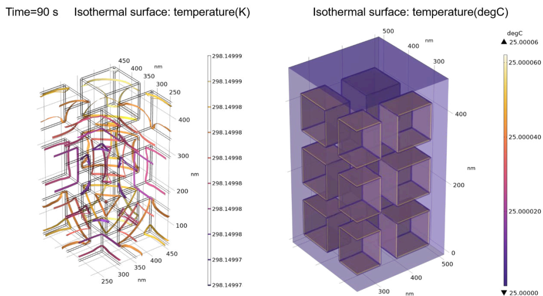
Fig. S15 Radiometric heat map of BGA. (a) Isothermal surface. (b) Body surface temperature.
