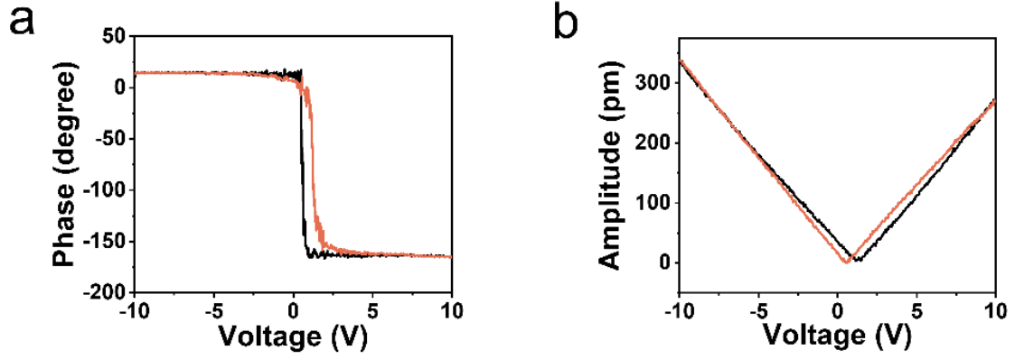
Fig. S11 (a) phase lag loop, (b) amplitude butterfly loop of BGA.
