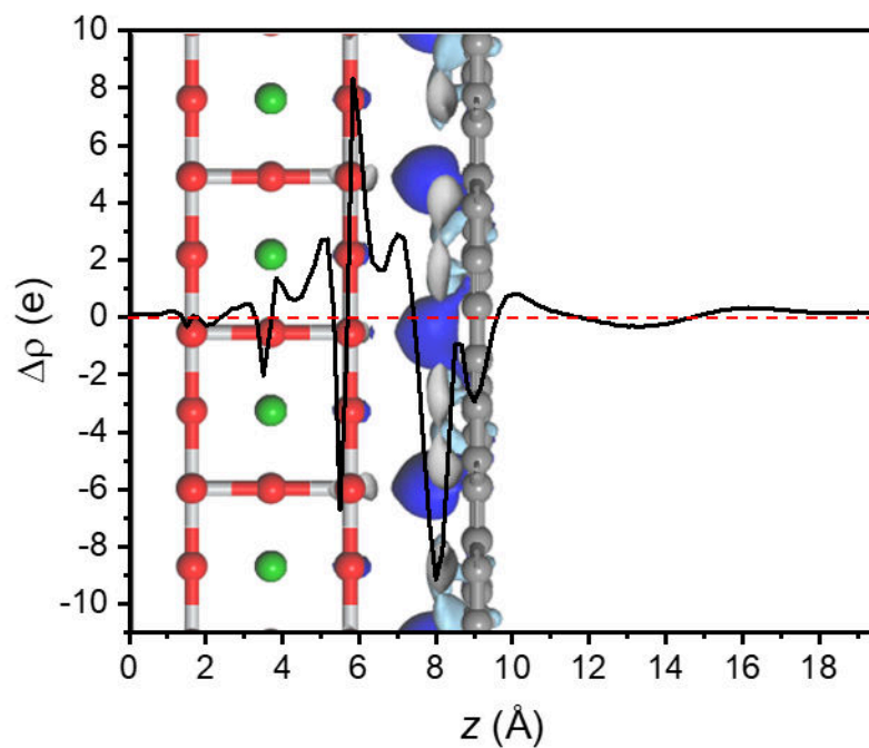
Fig. S13 Electron density difference plots for BGA and z-axis values of electron density difference and electron density difference plots of BGA in stretching (left) or compression (right), where positive and negative values represent electron gains and losses.
