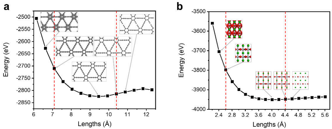
Fig. S12 The horizontal coordinate is the lattice constant of the cell, the vertical coordinate is the total energy of a single cell, and the red line is the range between (a) GDY, and (b) BTO for the stable existence of the cell.
