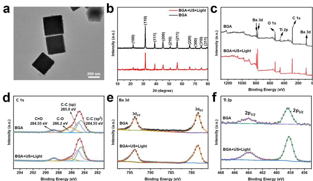
Fig. S8 (a) TEM image of BGA. (b) XRD patterns of BGA and BGA (US+Light). (c) XPS spectra of BGA, and BGA (US+Light), (d) C 1 s, (e) Ba 3d, and (f) Ti 2p.
