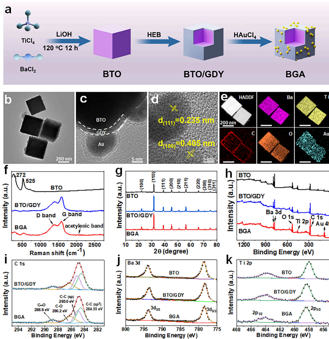
Fig. 1. Synthesis and characterization of BGA (a) Synthetic route, (b) (c) high magnification of TEM and (d) HRTEM images of BGA. (e) TEM image and EDS elemental maps of BGA. (f) Raman spectra of BTO, BTO/GDY, and BGA. (g) XRD patterns of BTO, BTO/GDY, and BGA. (h) XPS
