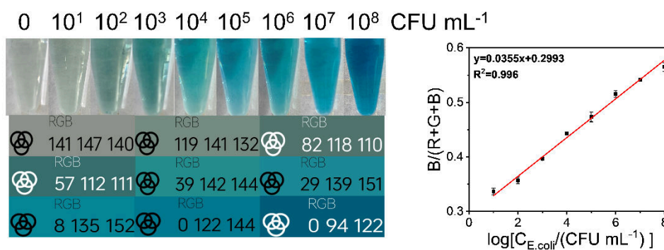
Fig.S16 Colorimetric method for detection of E. coli standard concentration color rendering diagram and corresponding B/(R+G+B) standard line.
