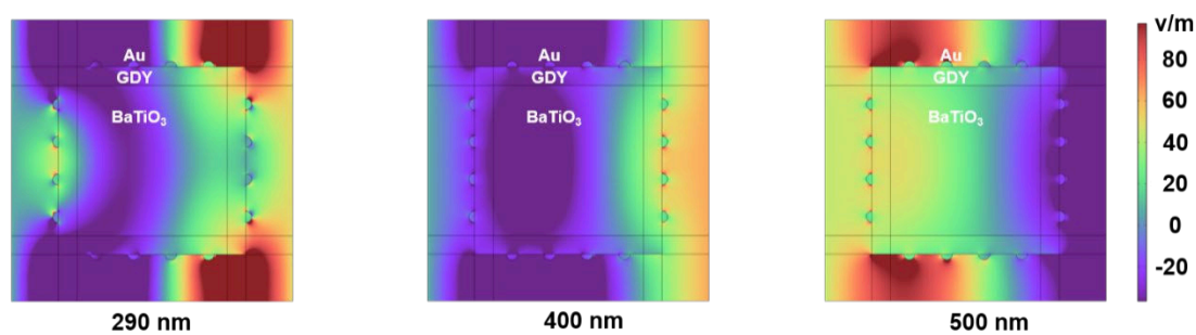
Fig. S14 Surface electric field distribution of BGA under different wavelengths of light.
