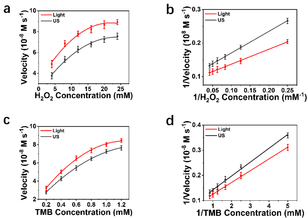
Fig. S7 Reaction kinetics curves of BGA under different external field conditions.
