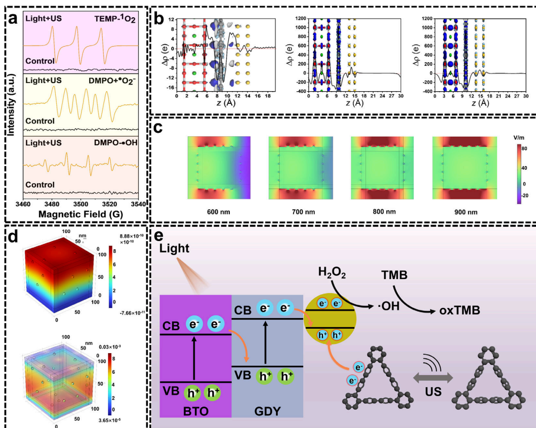
Fig. 3. (a) EPR spectra of TEMP- ^1\text{O}_2 adducts, DMPO- \cdot\text{O}_2^- , and DMPO- \cdot\text{OH} adducts. [DMPO]=[TEMP]=50 mM. (b) Electron density difference plots for BGA and z-axis values of electron density difference and electron density difference plots of BGA in stretching (left) or compression (right), where positive and negative values represent electron gains and losses. (c) Surface electric field distribution of BGA under different wavelengths of light. (d) Electric field diagram and Electric field diagram of BGA in z-axis US field of BGA. (e) Charge transfer pathways of BGA under light and US and their possible catalytic mechanisms.
