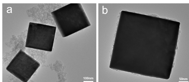
Fig. S1 TEM images of the (a)BTO and (b)BTO/GDY.
