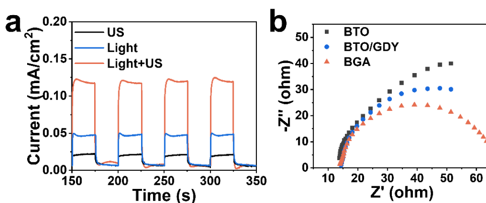
Fig. S10 (a) Piezoelectric and photocurrent response of BGA (b) EIS spectra of BTO, BTO/GDY, and BGA.
