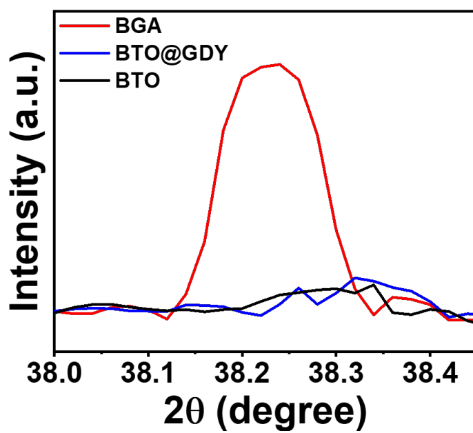
Fig. S2 XRD local enlargements of BTO, BTO/GDY, and BGA.
