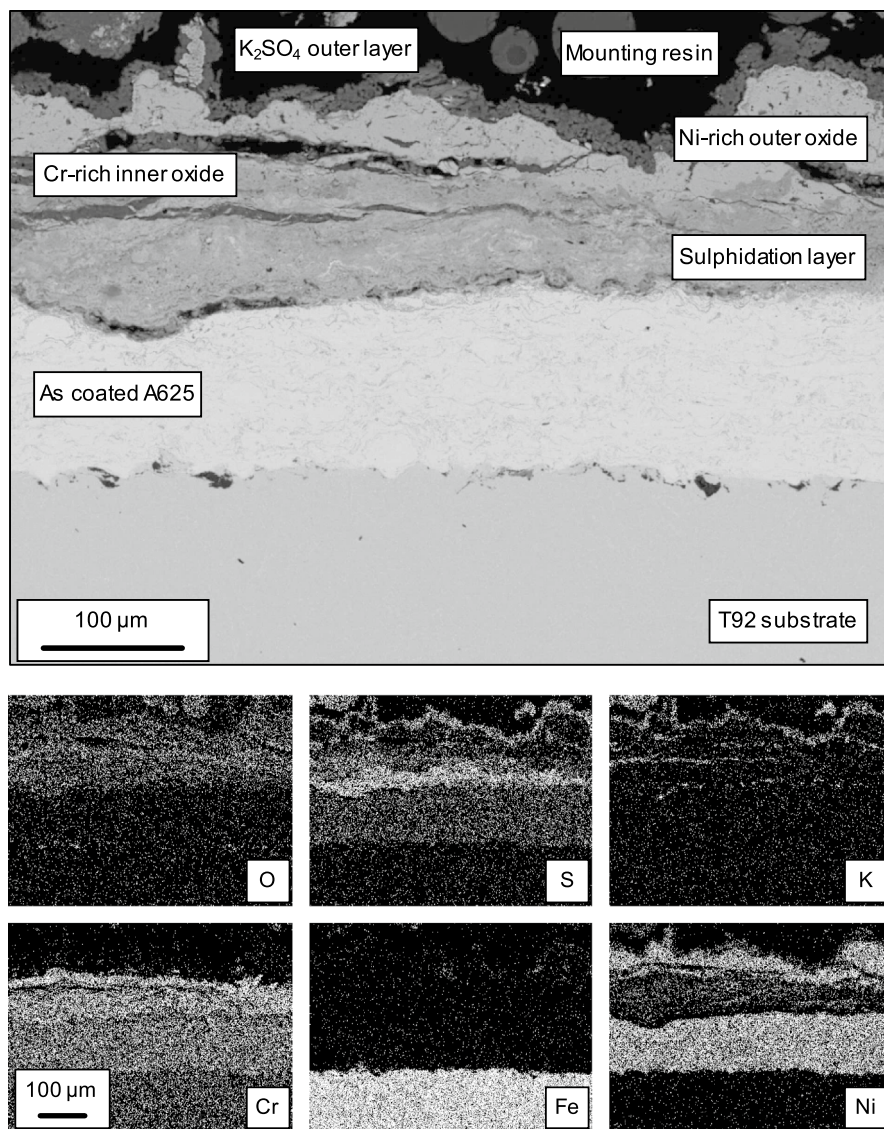
Fig. 7 BSE cross-section image and EDX maps of A625-coated T92 exposed to a simulated biomass environment at 600 °C for 1000 h
