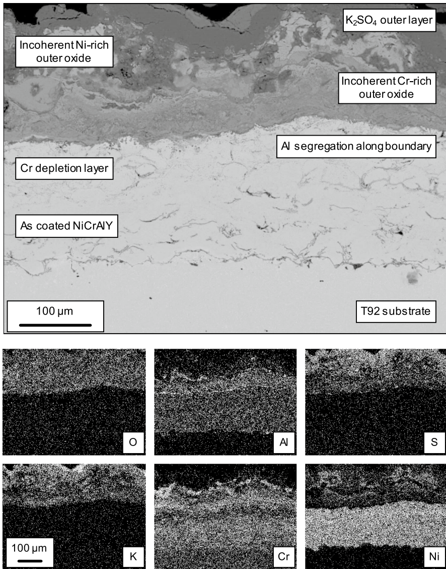
Fig. 8 BSE cross-section image and EDX maps of NiCrAlY coated T92 exposed to a simulated biomass environment at 600 °C for 1000 h
