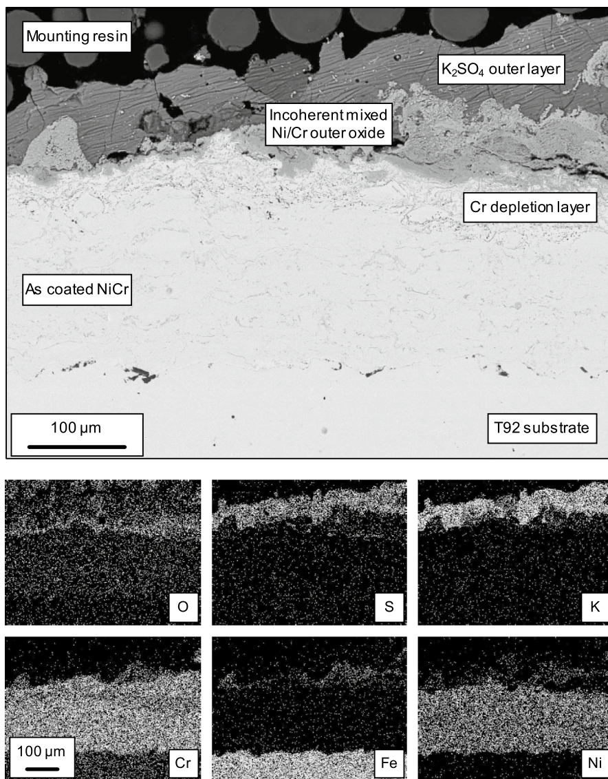
Fig. 9 BSE cross-section image and EDX maps of NiCr coated T92 exposed to a simulated biomass environment at 600 °C for 1000 h
