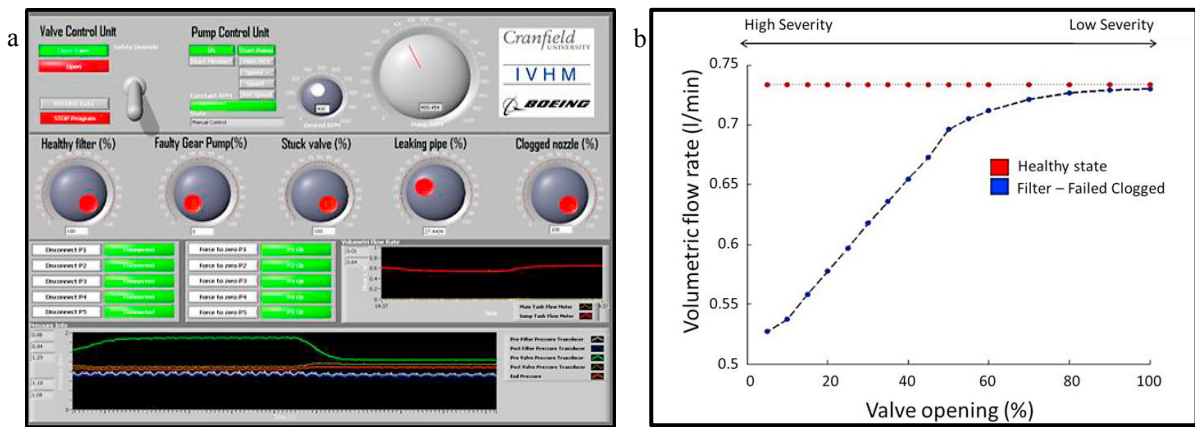
Fig. 5. (a) Fuel system – GUI for controls; (b) Output of simulated failure mode for a clogged filter vs. the healthy state.
