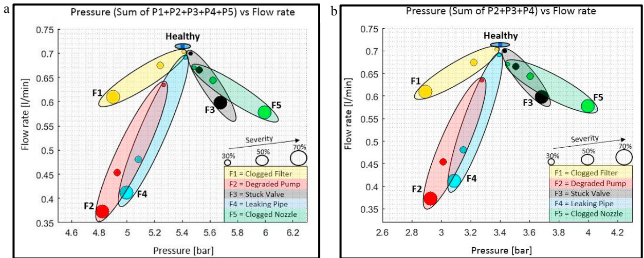
Fig. 7. (a) System Pressure (Sum of P1+P2+P3+P4+P5) vs Flow rate; (b) System Pressure (Sum of P2+P3+P4) vs Flow rate.
