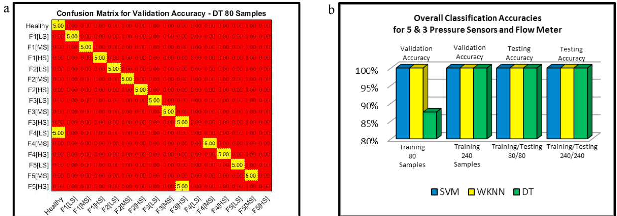
Fig. 8. (a) Confusion matrix for DT with 80 samples [19]; (b) Overall classification accuracies for 5 & 3 pressure sensors and flow meter.
