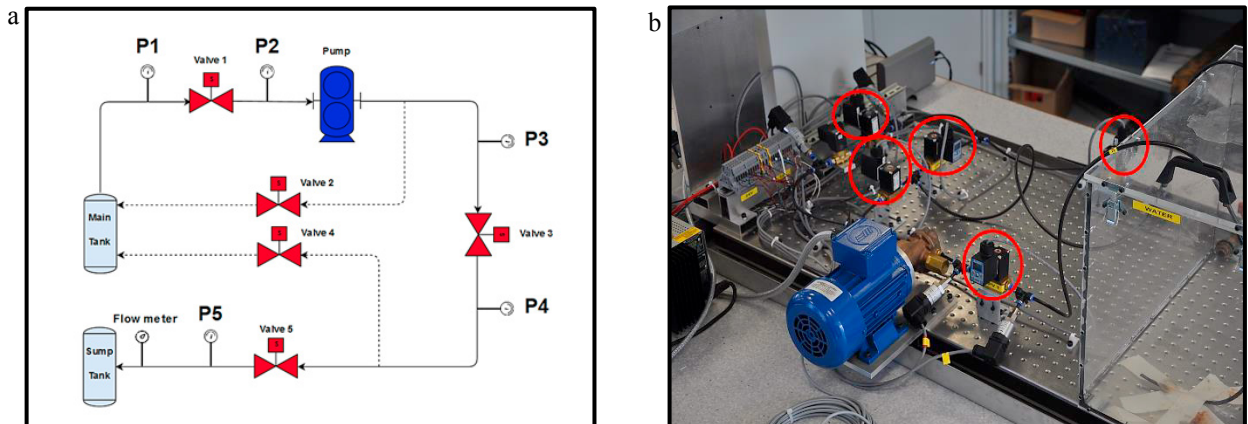
Fig. 4. (a) Schematic of modified fuel system; (b) Fuel system test rig.
