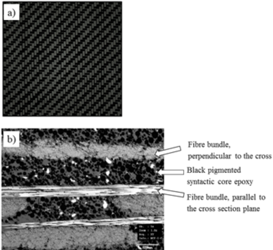
Figure1: a) The 2 x 2 twill weaving pattern of CF3500 woven carbon fibre ply. b) Microscopic image of cross section of cured VTS243FR/CF3500 composite; image scale shown on bottom right: 320 mm
