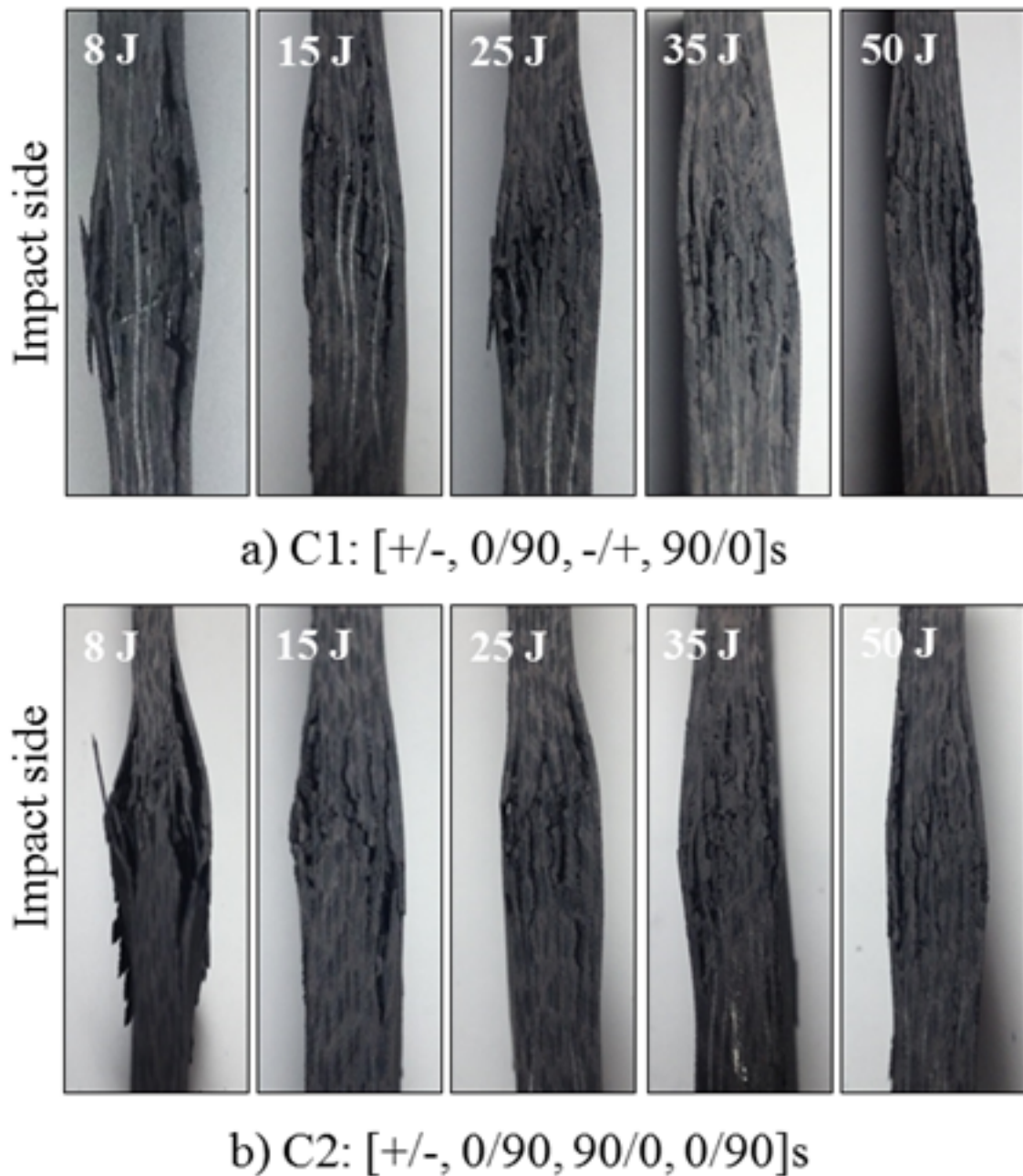
Figure 9: Photos of failed specimens after the CAI tests at various impact energy levels. “Pine tree” shaped fracture pattern clearly visible
