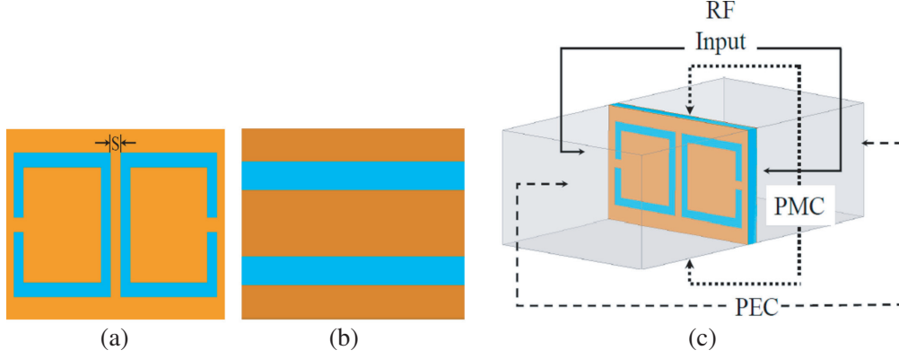
Figure 2. Unit cell simulation setup. (a) Top view. (b) Bottom view. (c) Simulation setup.
