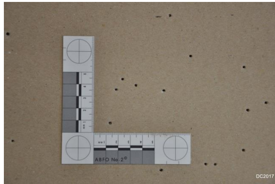
Figure 2. Typical strawboard (first layer, 1.4 m) after detonation of a M75 grenade.
