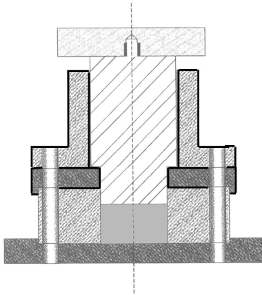
Figure 2 the Cranfield set-back simulator test vehicle
