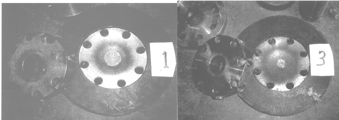
Figure 8 showing the base plates and confining rings for firings 1 (l) and 3(r). The first firing has run to detonation whereas the third firing is only a deflagration/ burn
