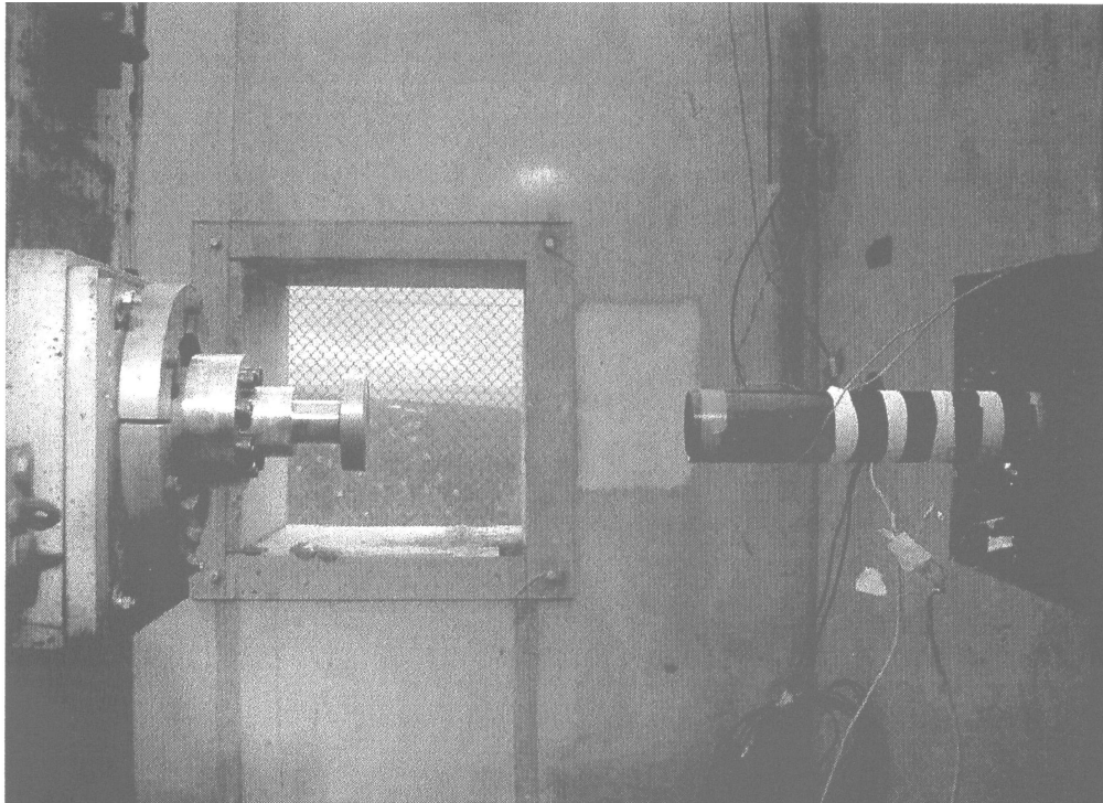
Figure 6 showing target assembly in front of velocity measuring tube attached to the gun barrel with the high speed video camera window
