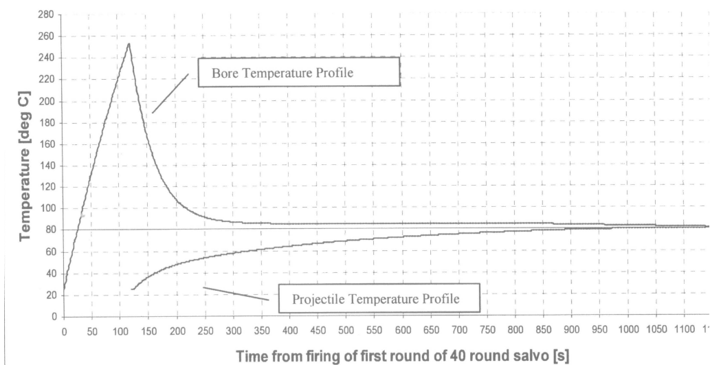
Figure 5 time temperature profile for a projectile and barrel in a hot gun scenario
