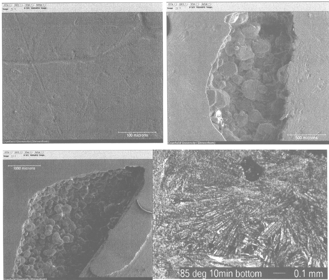
Figure 7 Electron Microscopy of composition B castings top left as cast top right 10 minutes anneal at 80 bottom left 15 minutes at 85°C and fragment after impact
