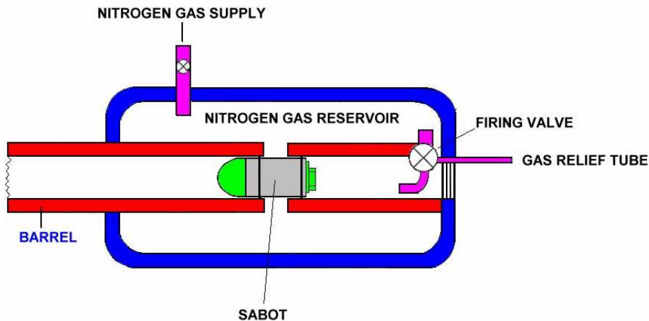
Figure 3 schematic of the compressed gas powered gun
