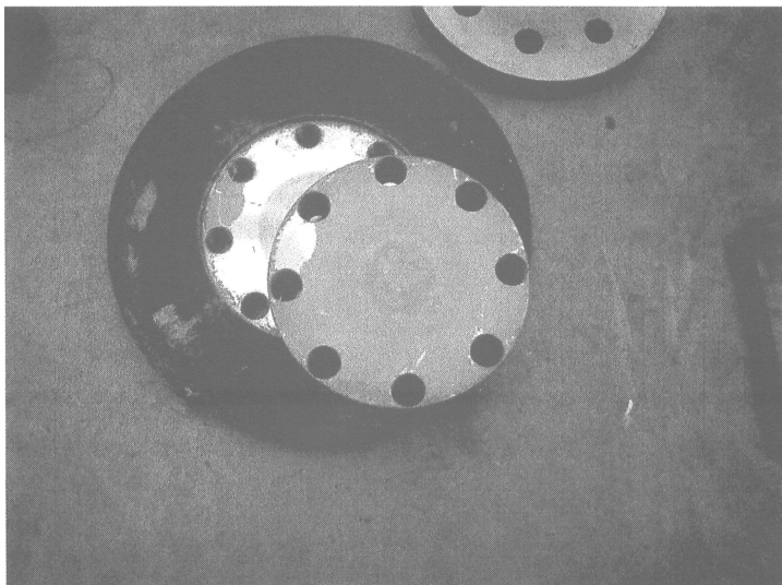
Figure 9 showing the hydraulic squeezing of the composition B filling between the base plate and the confining ring with no ignition evidence apart from a slight odour.
