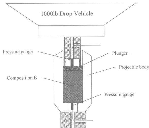
Figure Schematic of the NSWC setback simulator
