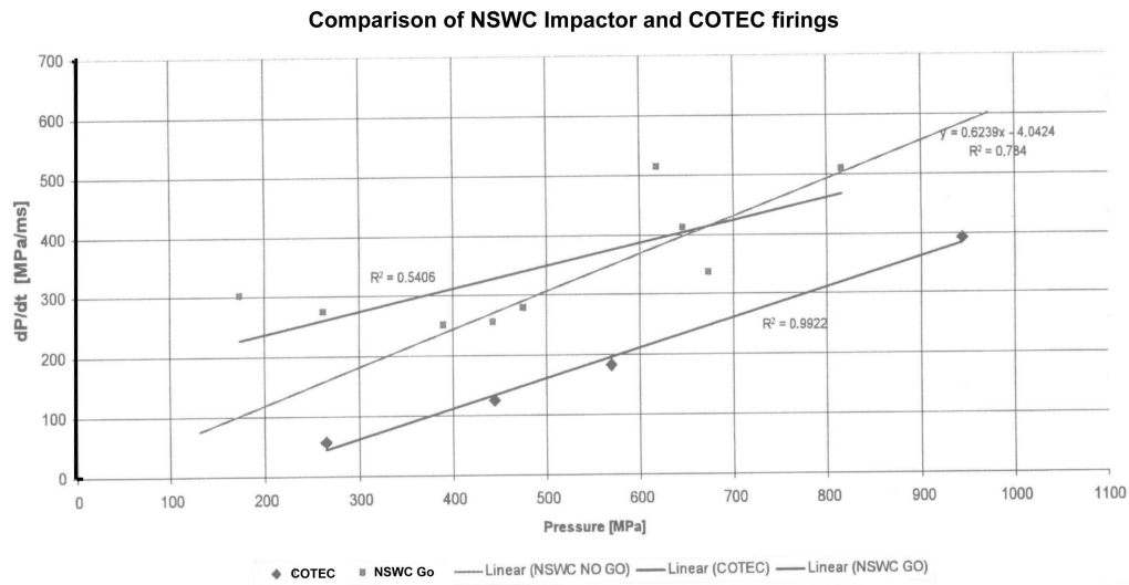
Figure 10 Comparison of NSWIC and COTEC results for Composition B
