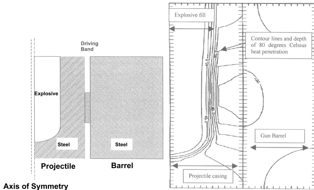
Figure 4 Area of contact between projectile and Barrel and the depth contour lines for the 80oC heat penetration as a function of time
