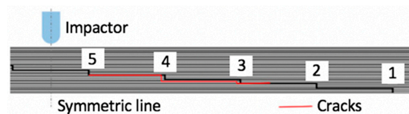
Figure 3. Location of cracks from 10 J impact performed by Liu et al. [24].
