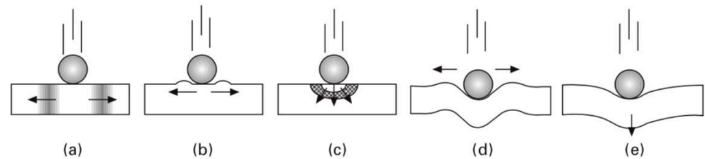
Figure 1. Wave shapes discussed by Olsson [11]: (a) fast tensile or compressive waves in the plane of the laminate, (b) fast surface waves along the laminate surface, (c) somewhat slower tensile or compressive waves through the thickness of the laminate, (d) relatively slow transient shear and flexural waves within the laminate, and (e) slow oscillation involving global quasi-static deflection.
