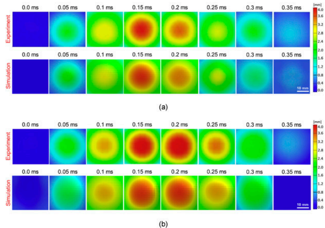
Figure 4. The out-of-plane displacement traces of high-velocity impacts on woven carbon-fibre/PEEK samples from experimental and numerical work for (a) a gelatine projectile, and (b) a HDPE projectile by Liu et al. [48].
