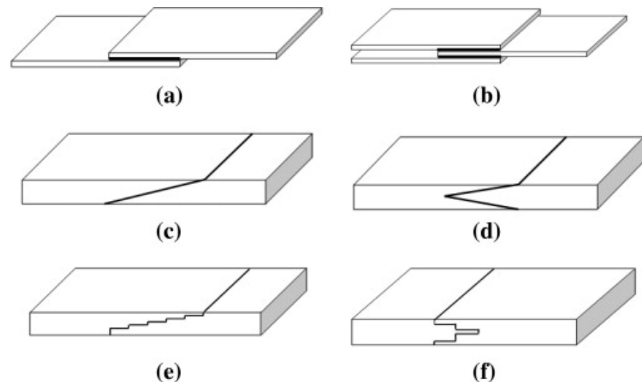
Figure 2. Types of adhesive joints shown by Kiniaiefar et al. [14]: (a) single lap joint, (b) double lap joint, (c) scarfed lap joint, (d) double sided scarfed joint, (e) stepped lap joint, and (f) double sided stepped lap joint.
