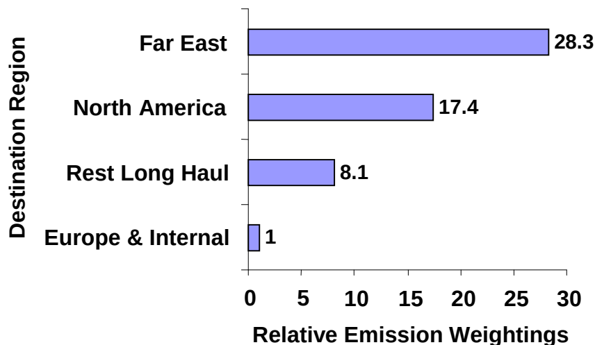
Figure 3. Relative Emission Weightings (calculated from 'Pagoda' data in Graichen and Guegle, 2006).
