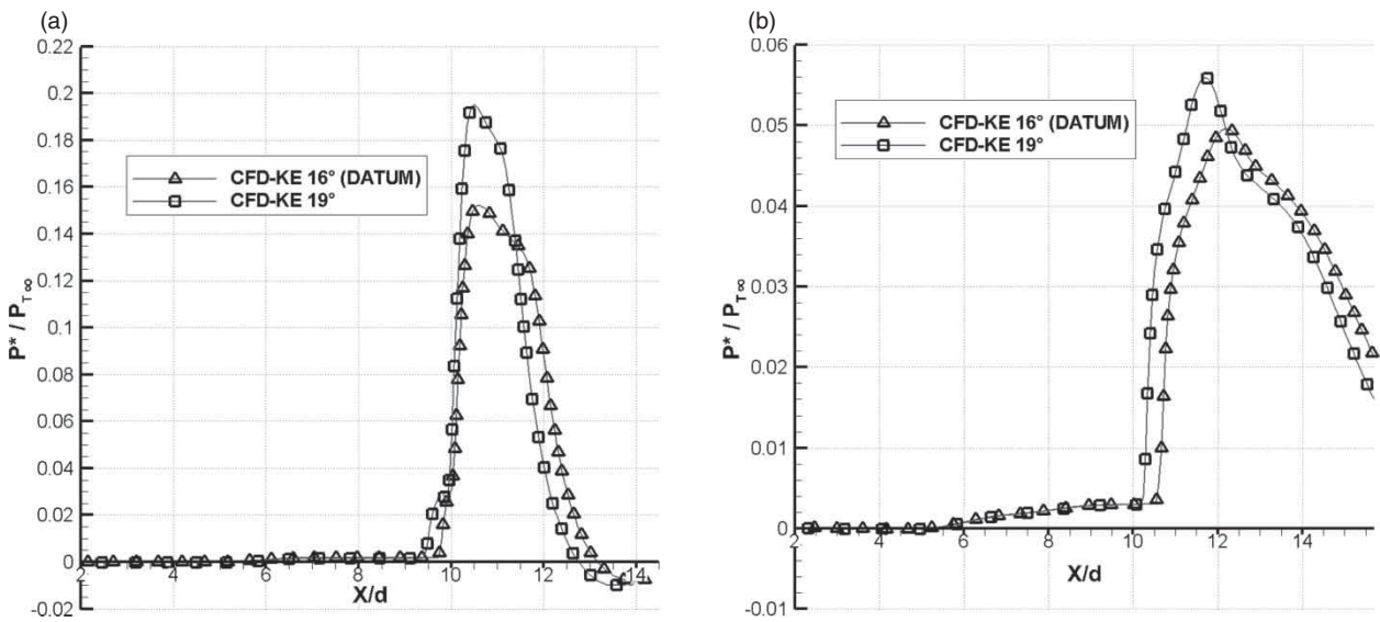
Figure 13. (a) Windward ( \phi = 0^\circ ) and (b) leeward ( \phi = 180^\circ ) surface pressure plot comparing k-\epsilon model at \alpha = 16^\circ and \alpha = 19^\circ at every \sim 10^{th} data point. 3M mesh. M = 2.88 , Re_L = 18.2 \times 10^6 , T_{T\infty} = 278 K, P_{T\infty} = 172.4 kPa.
