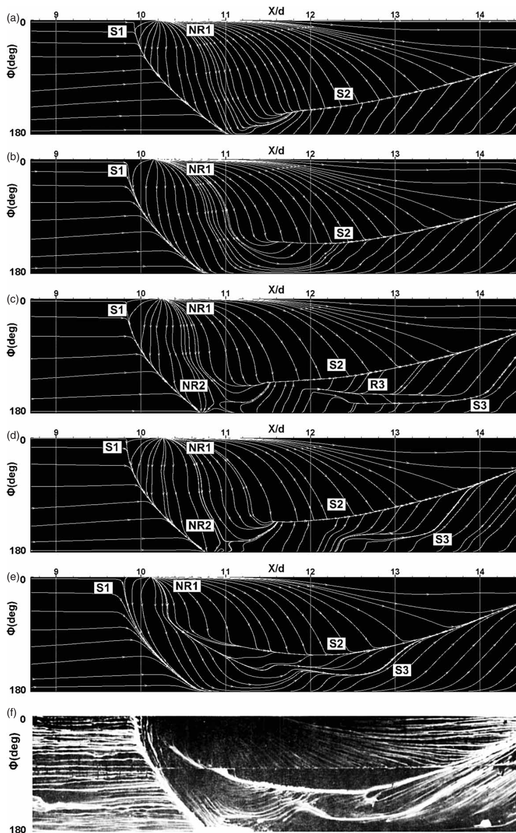
Figure 7. Comparison of computational streamlines, with experimental Mylar oil flow visualisation (a) SA, (b) k-\epsilon , (c) SST, (d) tSST, (e) RSM. M = 2.88 , \alpha = 16^\circ , Re_L = 18.2 \times 10^6 , T_{T\infty} = 278 K, P_{T\infty} = 172.4 kPa. Figure 7(f): This figure is taken from NASA-TM-84410, 'An Experimental Investigation of the Impingement of a Planar Shock Wave on an Axisymmetric Body at Mach 3', by A. Brosh, M. Kussoy, and used with permission of NASA.
