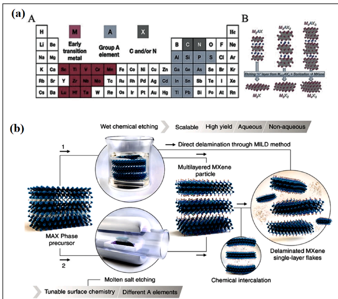
Fig. 2. (a) A representative of Elements involved in the formation of MAX phase and B representative of MXenes derived from different MAX phases [30], (b) Typical intercalation process in MXenes, emphasising the significance of this technique in tuning properties through synthesis conditions, intercalation, and post-processing [28].
