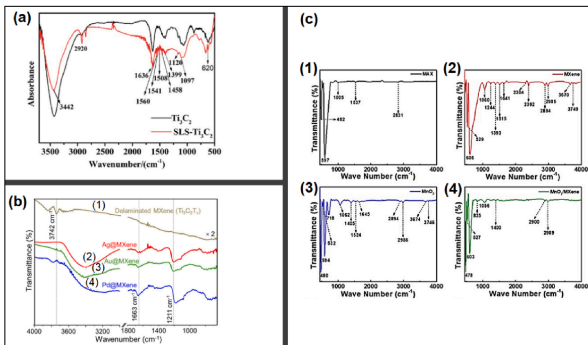
Fig. 6. (a) The FTIR spectra of \text{Ti}_3\text{C}_2\text{T}_x with and without sodium lignin sulfonate (SLS) functionalisation [188], (b) The ATR-FTIR spectroscopy (1) delaminated MXene nanosheets ( \text{Ti}_3\text{C}_2\text{T}_x ), as well as (2) Ag@, (3) Au@, and (4) Pd@MXene hybrids [181], (c) The Fourier-transform infrared (FTIR) spectra of (1) MAX powder, (2) exfoliated MXene, (3) \text{MnO}_2 nanowires (NWRs), and (4) \text{MnO}_2/\text{MXene} composite [187].
