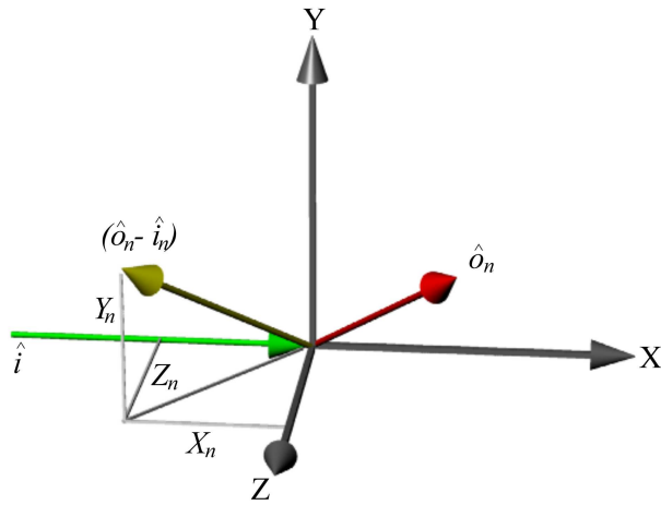
Figure 2. Definitions used in the conversion from measured velocity components to the orthogonal components. Here \hat{o}_n is the observation direction of the nth view and \hat{i} is the laser illumination direction; X_n , Y_n and Z_n are the Cartesian components of the measured velocity (\hat{o}_n - \hat{i}) component.
