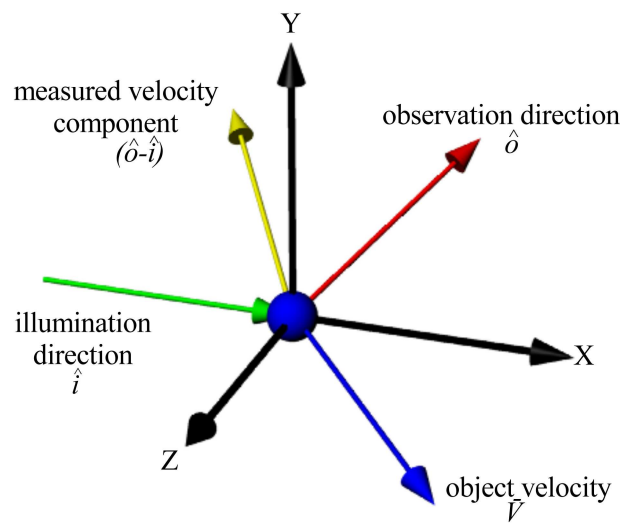
Figure 1. The relationship of laser illumination direction and observation direction to the measured velocity component determined from the Doppler equation. Here \hat{o} is the observation direction, \hat{i} is the laser illumination direction
