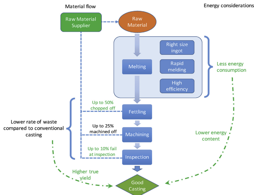
Fig. 6. Material and energy flow chart of a CRIMSON sand casting process.
