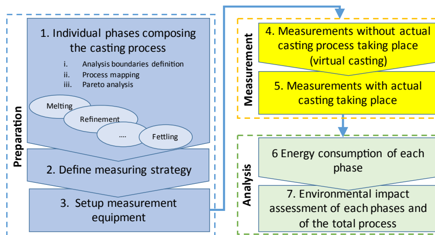
Fig. 1. Energy consumption measurement framework.
