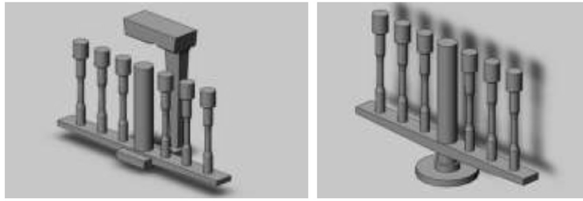
Fig. 7. Tensile bar casting system used (left) in gravity sand casting and (right) counter-gravity (up casting) CRIMSON sand casting process.
