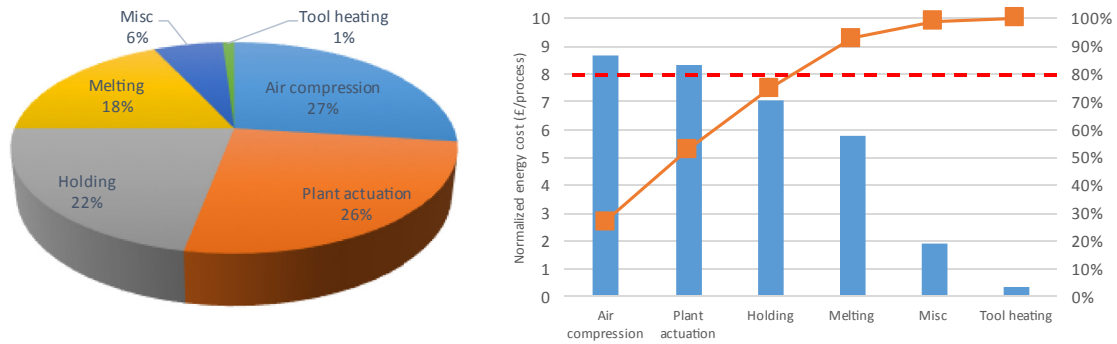
Fig. 3. (a) Energy cost (based on figures presented by DETR, 1997) and (b) Pareto analysis.
