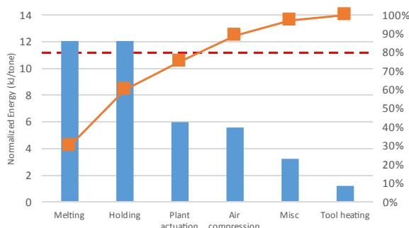
Fig. 2. (a) Typical energy use (based on figures presented by DETR, 1997) and (b) Pareto analysis.
