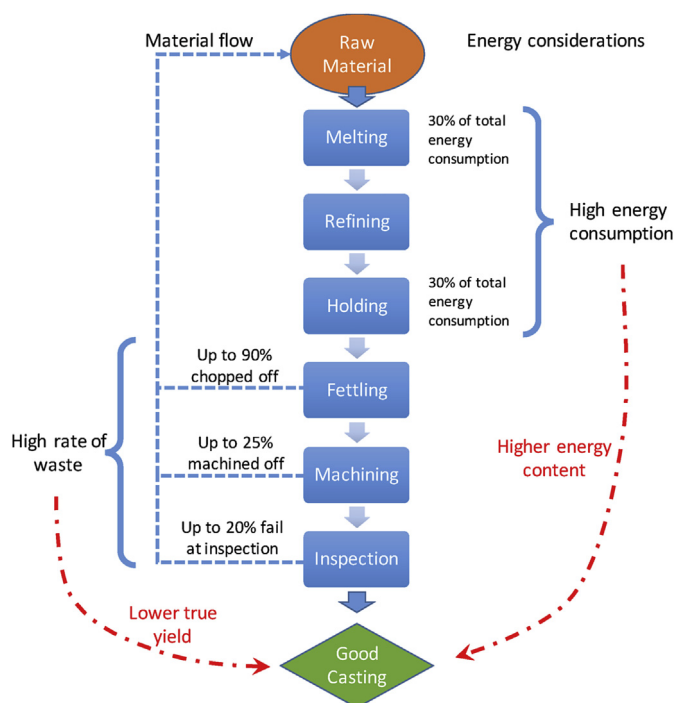
Fig. 5. Material and energy flow chart of a conventional sand casting process.
