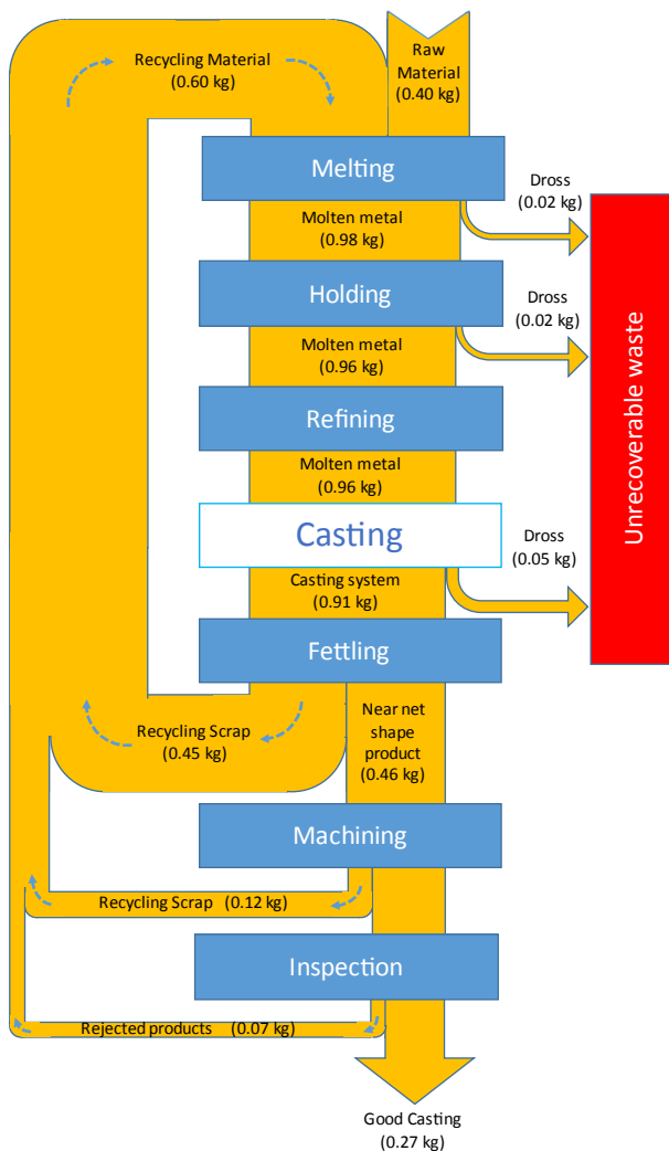
Fig. 4. Metal flow in the foundry.
