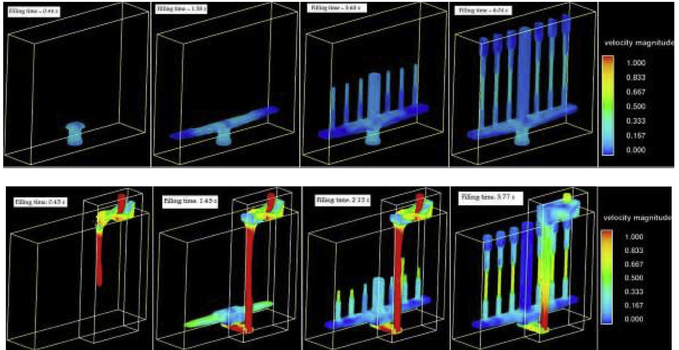
Fig. 8. Numerical simulation of runner system of tensile bar for CRIMSON (up) and conventional sand casting process (down).
