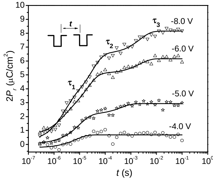
FIG. 2. Time dependence of remanent polarization under a negative voltage pulse sequence (inset) separated with relaxation time t under different V_{app} for PNZST. The pulse width is 100 ns. The solid lines are the best fitting of the data according to Eq. (5).
