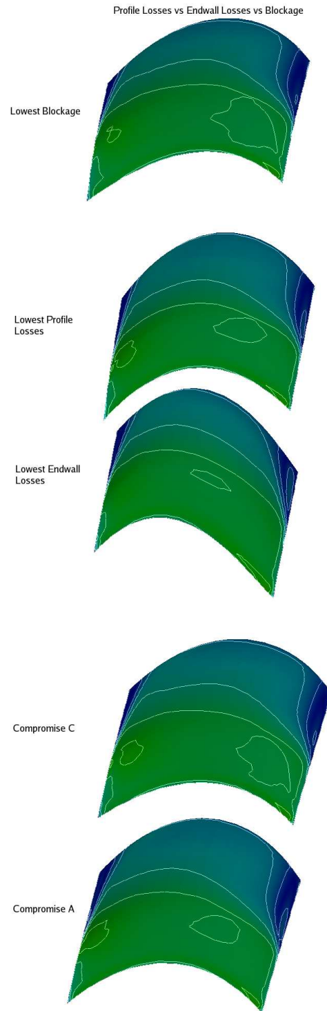
Figure 27 : The velocity contours for various optimal designs the test case 2
