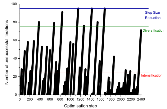
Figure 30 : The optimization search pattern for test case 2, shown through the number of consecutive unsuccessful iterations
