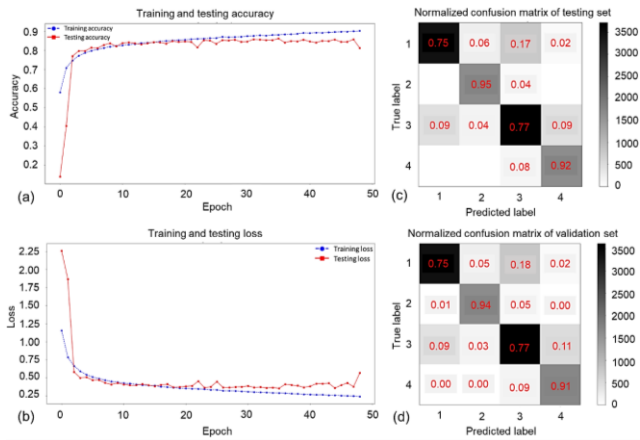
Fig. 10 The training, testing, and validation results of the Experiment A1 hyperparameter of BSF features. (a) refers to the training and testing accuracy chart, (b) refers to the training and testing loss chart, (c) refers to the normalized confusion matrix of the testing set, and (d) refers to the normalized confusion matrix of the validation set. The solid red lines in (a) and (b) refer to the testing process, while the blue dashed lines in (a) and (b) refer to the training process. The color bars in (c) and (d) refer to the number of samples.
