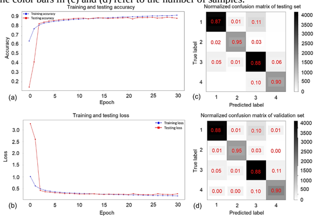
Fig. 11 The training, testing, and validation results of the Experiment A2 hyperparameter of BSF features. (a) refers to the training and testing accuracy chart, (b) refers to the training and testing loss chart, (c) refers to the normalized confusion matrix of the testing set, and (d) refers to the normalized confusion matrix of the validation set. The solid red lines in (a) and (b) refer to the testing process, while the blue dashed lines in (a) and (b) refer to the training process. The color bars in (c) and (d) refer to the number of samples.
