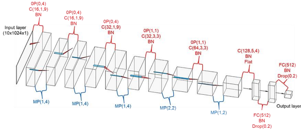
Fig. 5 The ConvNet classifier for flow regime classification. The grey cubes refer to the tensors. The blue cubes refer to the filter spaces. The red rectangular pyramids refer to the convolution or max-pooling layers, which are distinguished using red and blue texts. “ OP(w, h) ” refers to the zero-padding layer with the w \times h padding size, “ C(c, w, h) ” refers to the 2D convolutional layer with the w \times h convolutional kernel size and c channel, and “BN” refers to the batch normalization layer. “ MP(w, h) ” refers to the 2D max-pooling layer with w \times h kernel size. “FC( d )” refers to the fully connected dense layer with d nodes, “Flat” refers to the flatten layer, and “Drop( x )” refers to the dropout layer with dropout ratio x .
