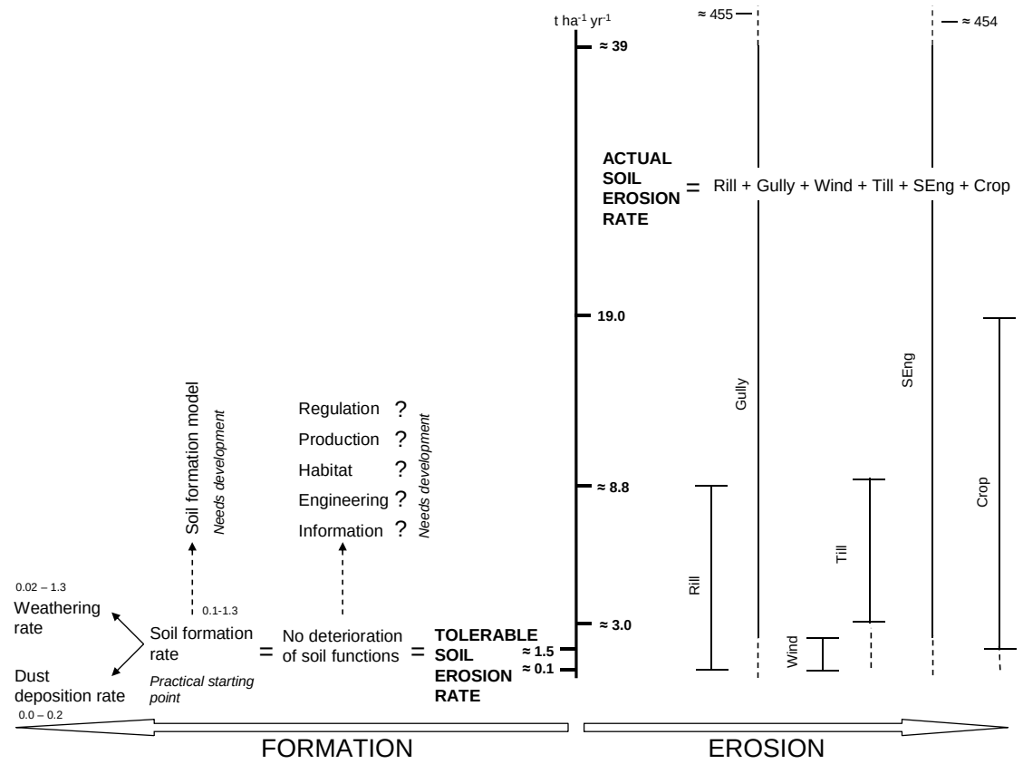
Tolerable vs. actual soil erosion, concept and rates. See the text for a detailed explanation. All numbers are in \text{t ha}^{-1} \text{yr}^{-1} . Please see relevant sections of this paper for more detailed information and references. Rill=rill and sheet erosion; Gully=gully erosion; Wind=wind erosion; Till=tillage erosion; SEng=erosion by slope engineering; Crop=erosion by crop harvesting.
