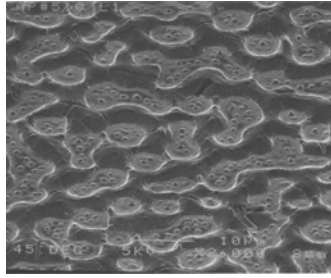
Figure 7: Surface of PZT thin film annealed with extended pulses of fluence 200\text{mJ}/\text{cm}^2 .
