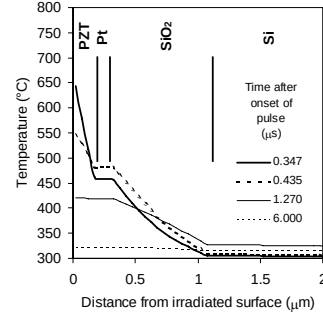
Figure 10: Modelled temperature distribution in layer stack with 300nm thick PZT thin film and extended laser pulse of fluence 100mJ/cm 2
