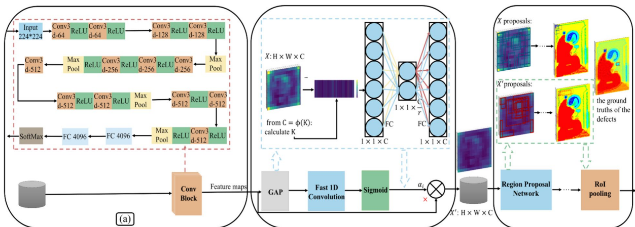
Fig. 7 a Original image input forward VGG16 network structure, b ECA module structure diagram, visualizing input feature map X and re-weighted output feature map X' c comparing the visualizations of X and X' proposals
