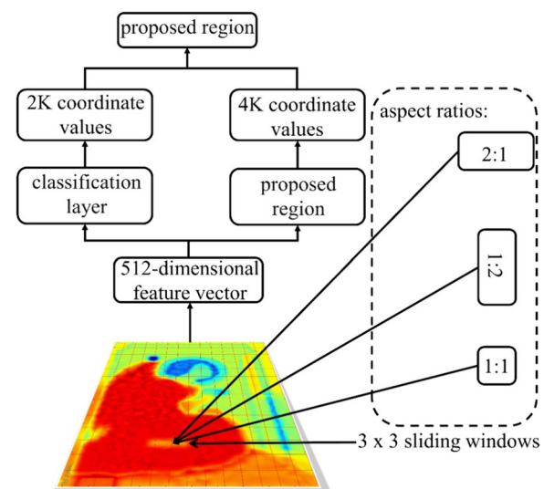
Fig. 6 RPN anchor frame structure diagram
