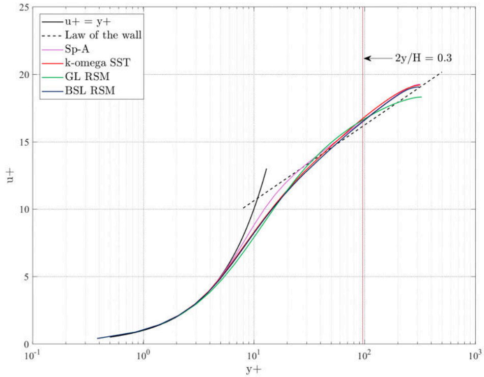
Figure 10: The figure shows half of the axial velocity profile in semi-log scale for different turbulence models together with the universal velocity profile.
