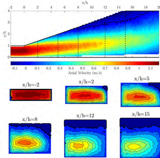
Figure 3: Velocity measurements in the Stanford diffuser. Top: Axial velocity contours on the central plane of the diffuser. Bottom: Axial velocity contours on cross-sectional slices along the diffuser. The black line marks the zero streamwise velocity contour [8].
