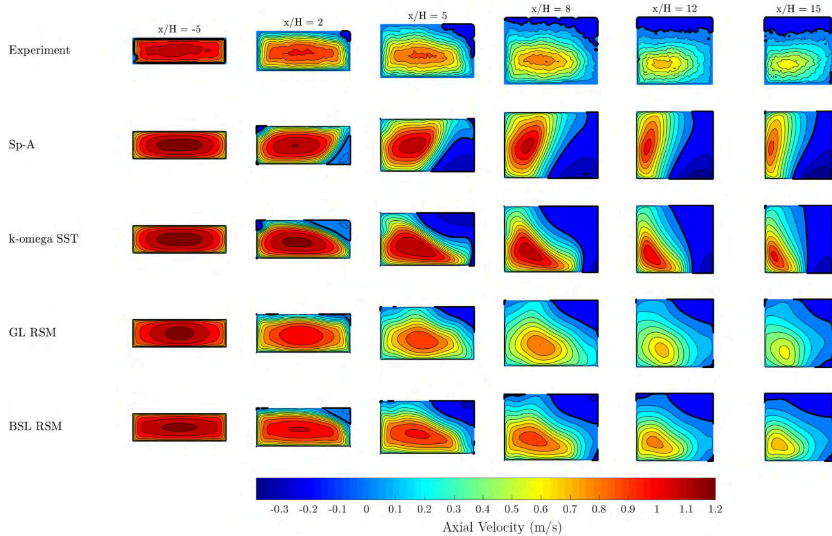
Figure 13: Streamwise velocity contours in the cross-plane z-y at six axial locations along the diffuser. The thick line marks the zero streamwise velocity contour. The dark blue areas are regions of reversed flow.
