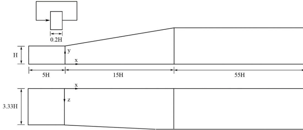
Figure 7: Schematic of the computational domain (diagram not to scale).
