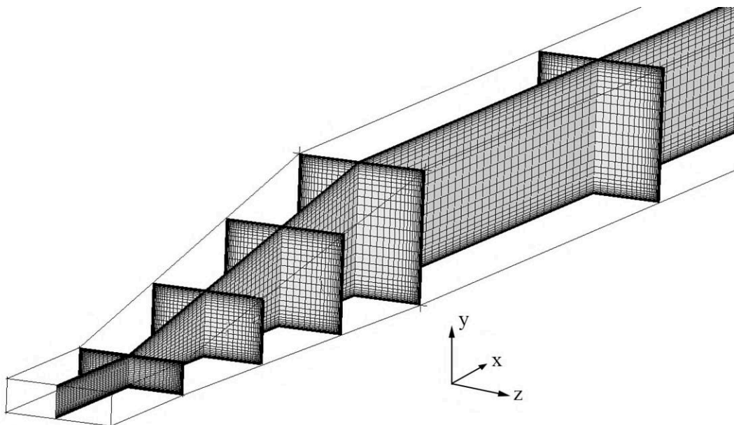
Figure 8: Grid distribution in the diffuser (medium grid).
