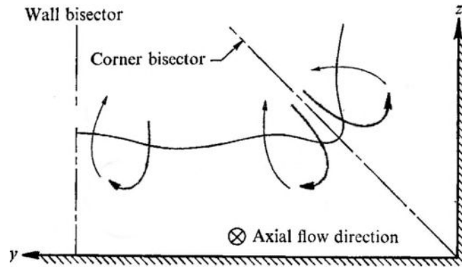
Figure 5: Contour of constant velocity pattern for flow near a corner [12].
