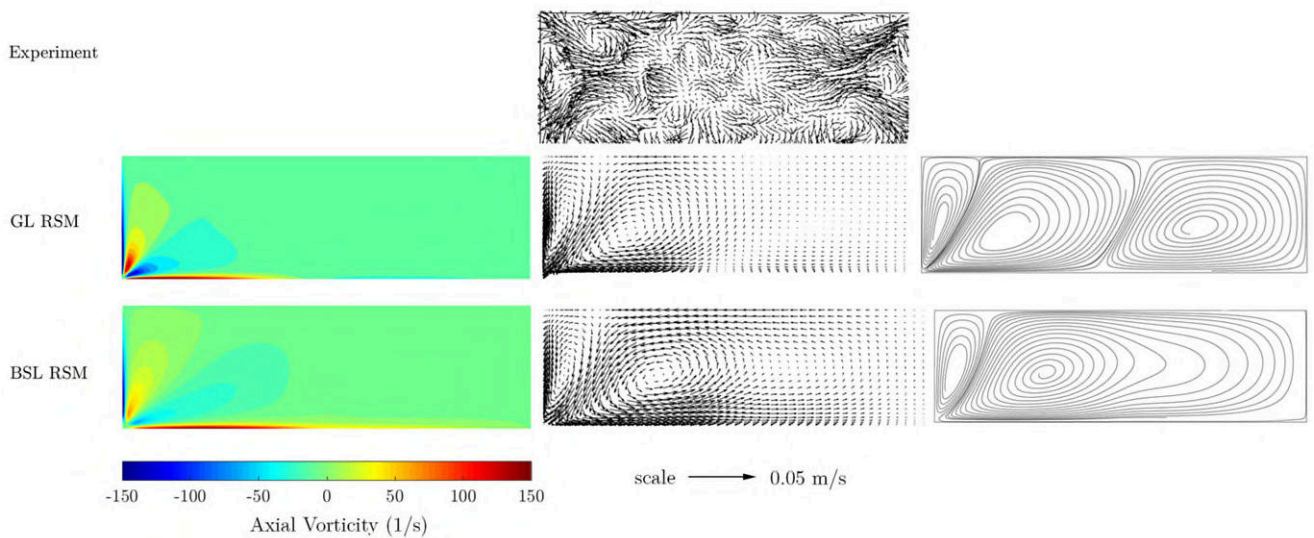
Figure 11: Turbulence-induced secondary flow in the inflow duct: plots of axial vorticity (left), in-plane velocity vectors (middle) and 2-D streamlines (right). The jet of high momentum fluid bisects the corner at approximately 45^\circ .
