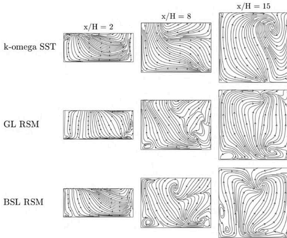
Figure 15: Streamlines of secondary flow (velocity in the z - y plane of the diffuser) at three streamwise locations predicted with the k - \omega SST, GL RSM and BSL RSM turbulence models.
