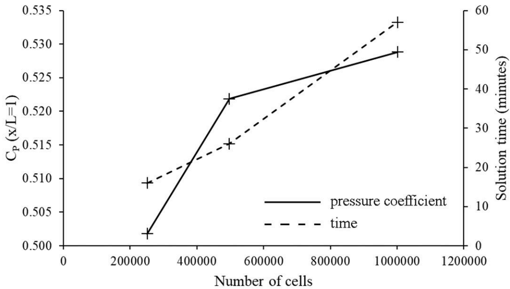
Figure 9: Grid convergence study for the periodic duct. The convergence of the pressure coefficient at x/L = 1 (solid line) was monitored together with the computational time (dashed line).
