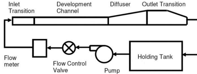
Figure 2: Schematic diagram of the experimental flow system [10].
