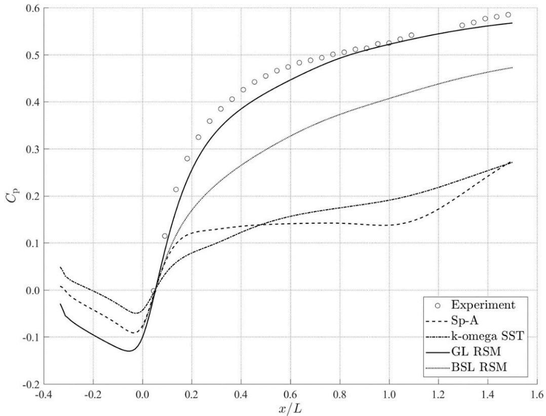
Figure 14: Recovery of pressure coefficient along the bottom wall of the diffuser. The reference pressure is the pressure at x/H = 0.05 and z/B = 0.5 . The length of the diffuser is L = 15 cm.
