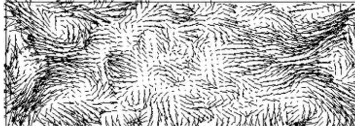
Figure 4: Experimental secondary flow currents in the inflow duct of the diffuser [8].
