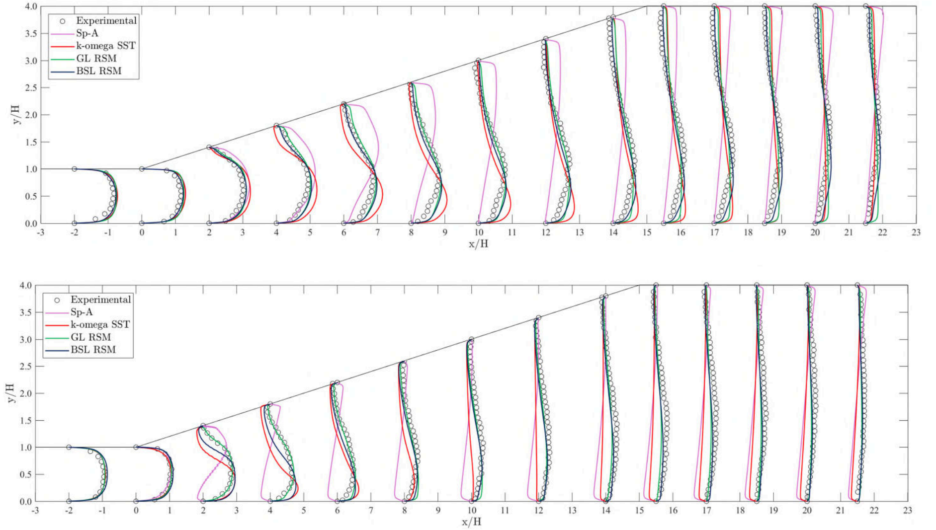
Figure 12: Development of axial velocity in the vertical plane for different turbulence models at spanwise locations of z/B = 1/2 (top) and z/B = 7/8 (bottom).
