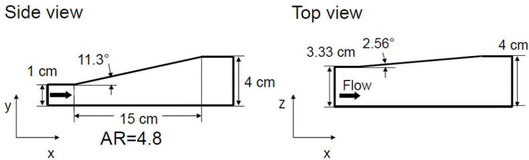
Figure 6: Geometry and dimensions of the test-case diffuser [10].
