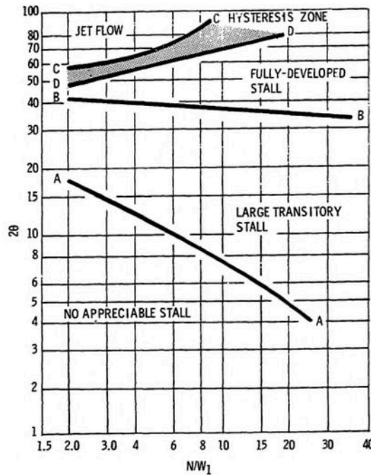
Figure 1: Flow regimes in 2-D diffusers [5].
