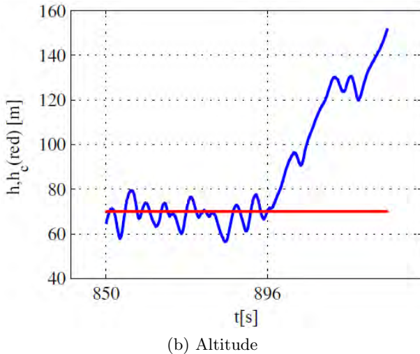
Fig. 9. Performance of the adaptive baseline under large uncertainties.
