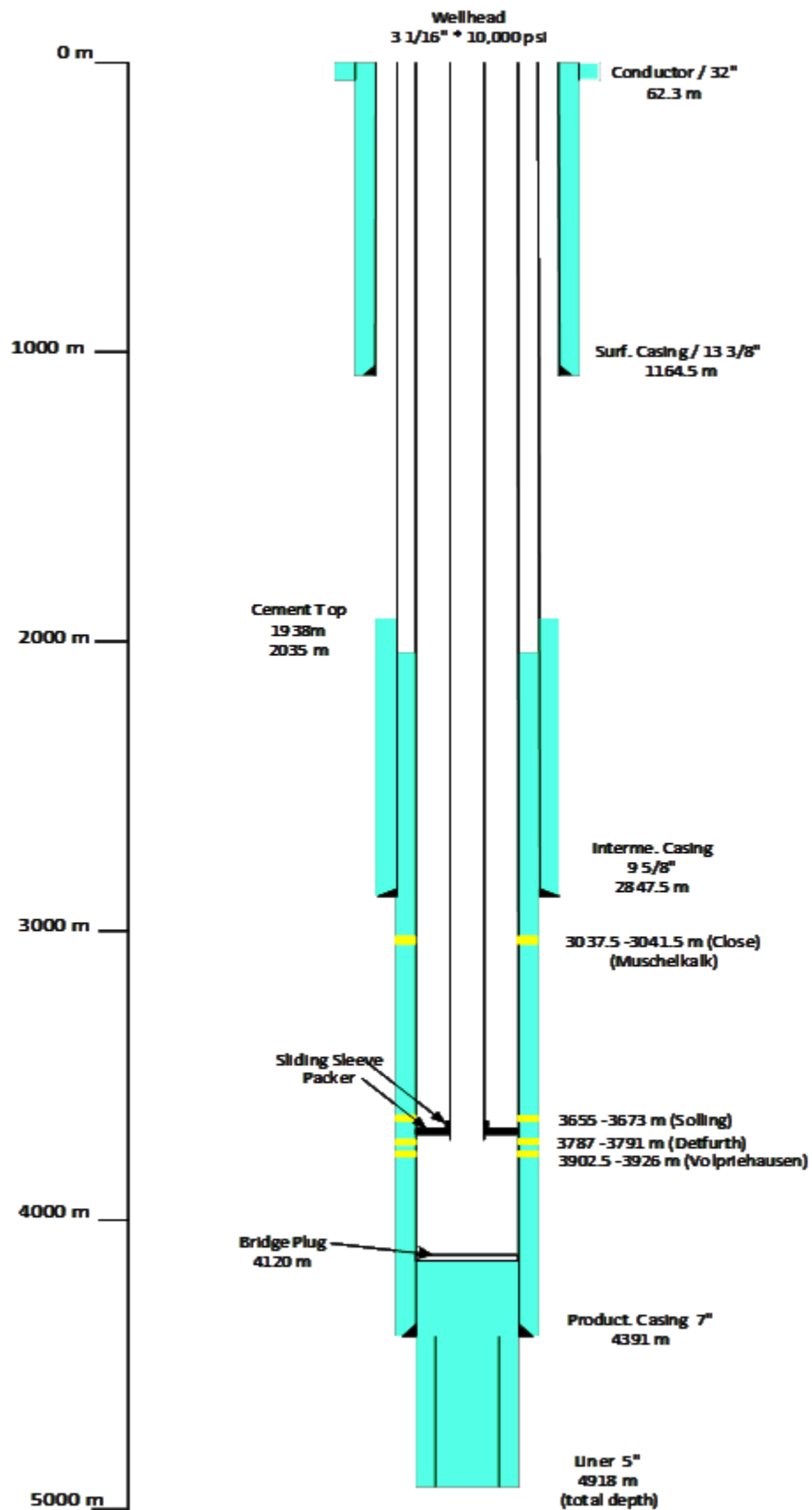
Figure 1 - Horstberg Z1 Well Schematic (Huenges and Ledru, 2010)
