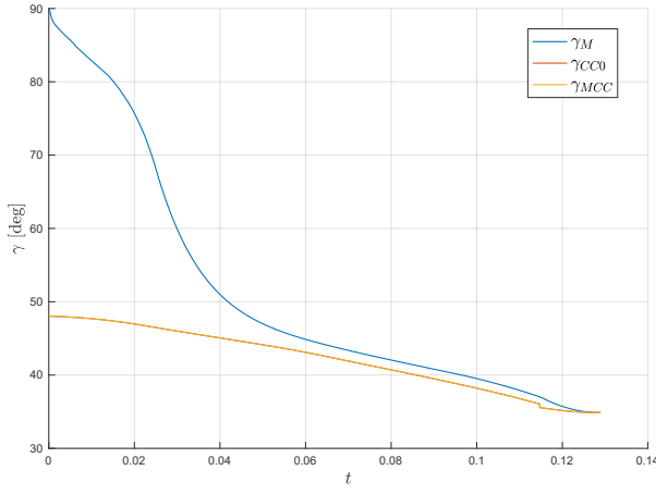
(a) Y_{T_0} = 0.1
