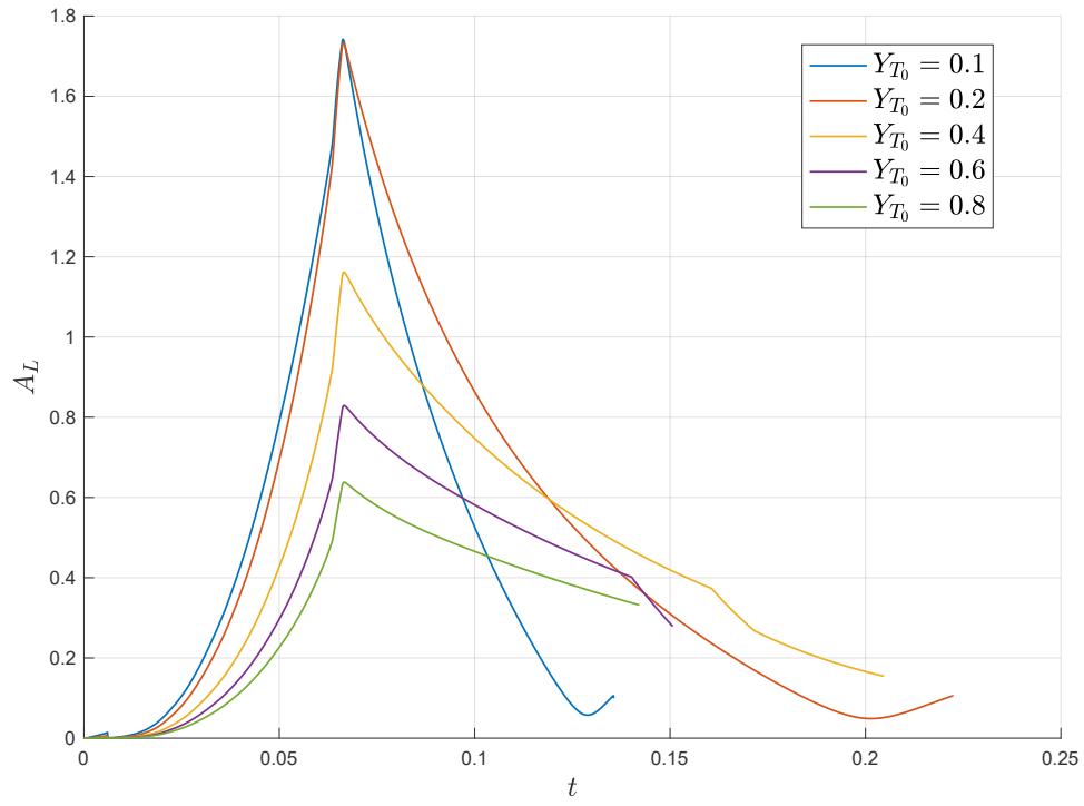
Fig. 24. Case 3. Lift Acceleration History for Pure PNG
