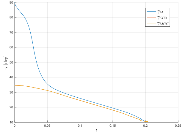
(b) Y_{T_0} = 0.2
