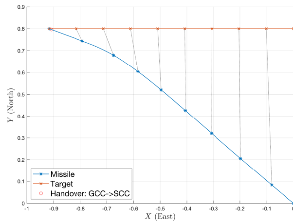
(e) Y_{T_0} = 0.8
