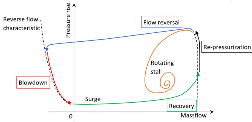
Figure 1 – Example of rotating stall and deep surge trajectories on the compressor map, with phases of surge highlighted.
