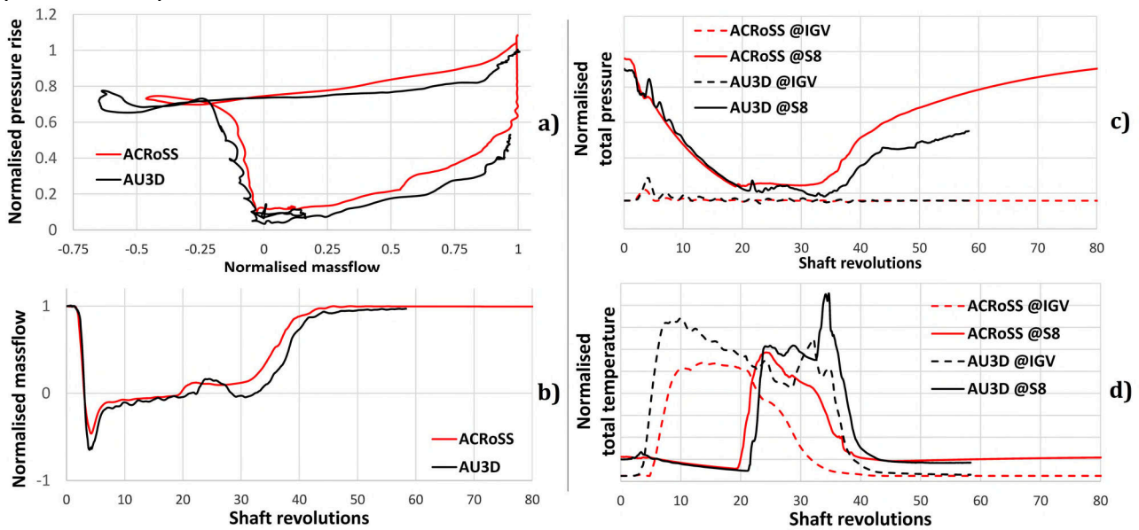
Figure 6 – Comparison of transient event time histories during surge at 85% speed from ACRoSS and AU3D. Compressor map a), massflow at IGV inlet (b), total pressure (c) and total temperature (d) at IGV inlet and stator 8 outlet.
