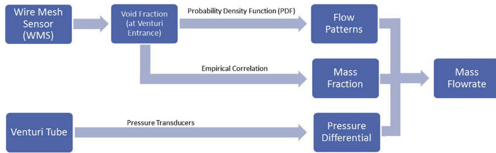
Fig. 4. Scheme of two-phase (air and water) flowrate measurements.
