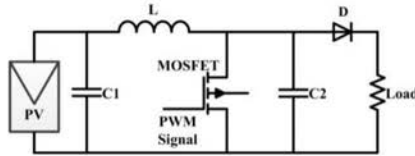
Fig. 3. Boost DC-DC converter
