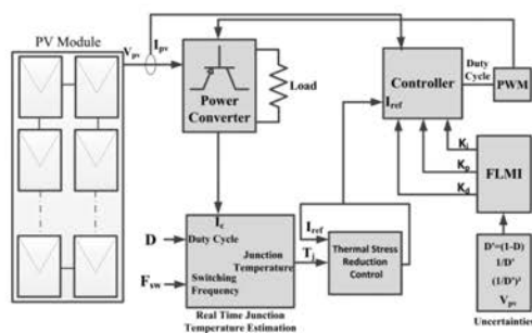
Fig. 1. Proposed schematic diagram of sensorless thermal stress reduction control.
