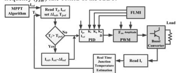
Fig. 2. Thermal stress reduction control strategy.
