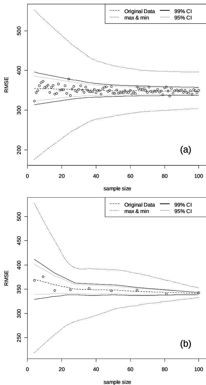
Figure 3. Example of the changes in the value of RMSE ( \mu\text{g kg}^{-1} ) from sample size 4–100 observed for DON for random (a) and regular (b) sampling strategies. The model was run to simulate a bulk commodity with mean DON concentration 7.14 ( \log_e 1260 \mu\text{g kg}^{-1} ) and a spatial distribution described by a variogram with range 4 m, sill 0.07 and nugget 0. The final simulated values were mean 6.5, range 3.66, sill 0.067 and nugget 0.0091.
