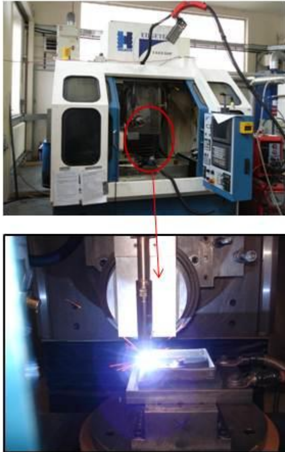
Fig. 4: Edgetek SAM machine integrated with CMT welding machine
