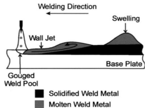
Fig. 2: Weld bead humping formation phenomenon (3)
