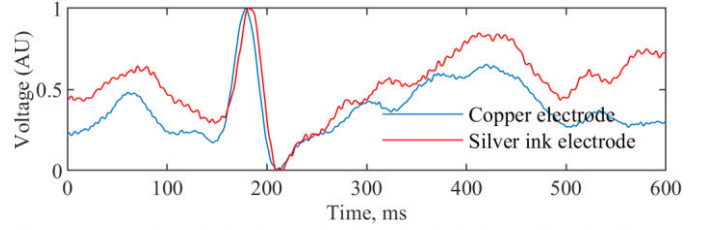
Fig. 10. Comparison of signal reproduction of a single human beat for silver conductive ink and copper electrodes
