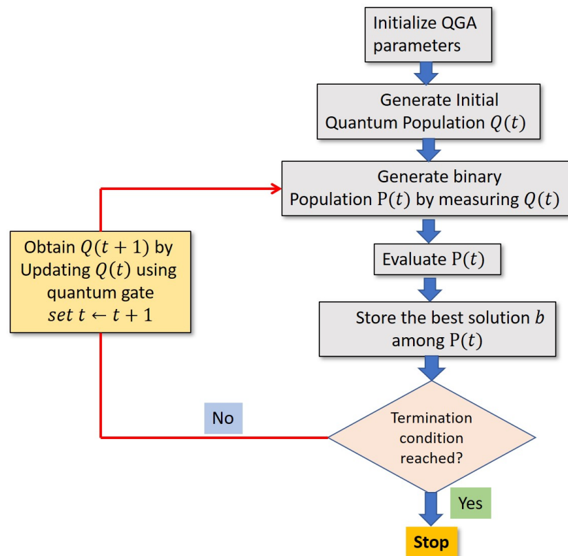
Figure 7. Flow diagram of 2D-QGA.
