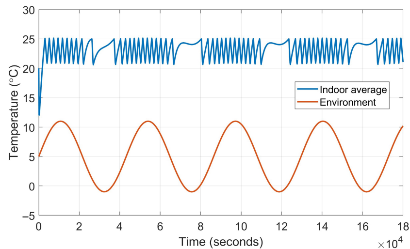
Figure 7. OpenADR-Enabled Scenario: Enhanced Indoor Comfort and Temperature Control Under Demand Response.
