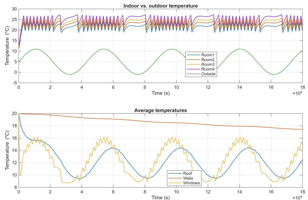
Figure 8. Room-Level and Building Envelope Temperature Profiles in OpenADR-Integrated Multi-Zone Heating System.
