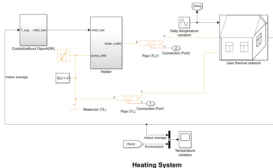
Figure 2. Layout of Scenario 1 on the simulation tool (without protocol).
