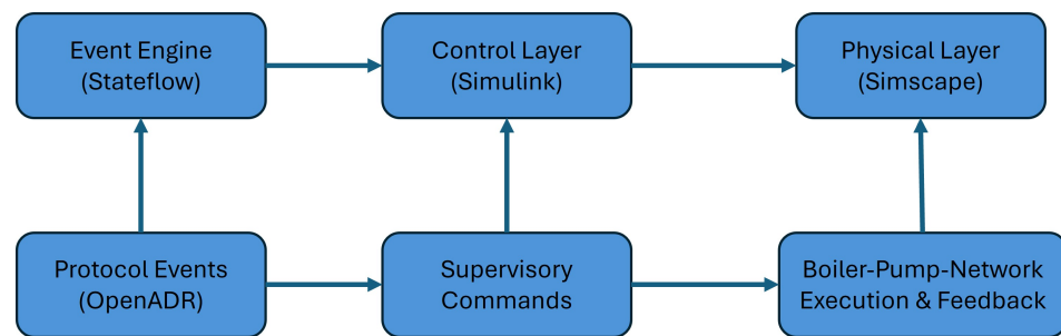
Figure 1. Protocol-driven simulation framework architecture for residential heating subsystem.
