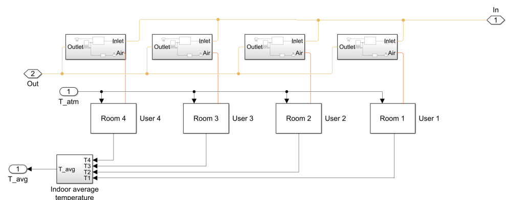
Figure 4. Layout of User thermal network.
