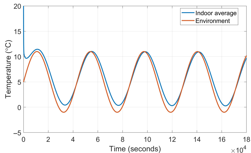
Figure 6. Baseline Scenario: Indoor and Outdoor Temperature Variation Without OpenADR Protocol.
