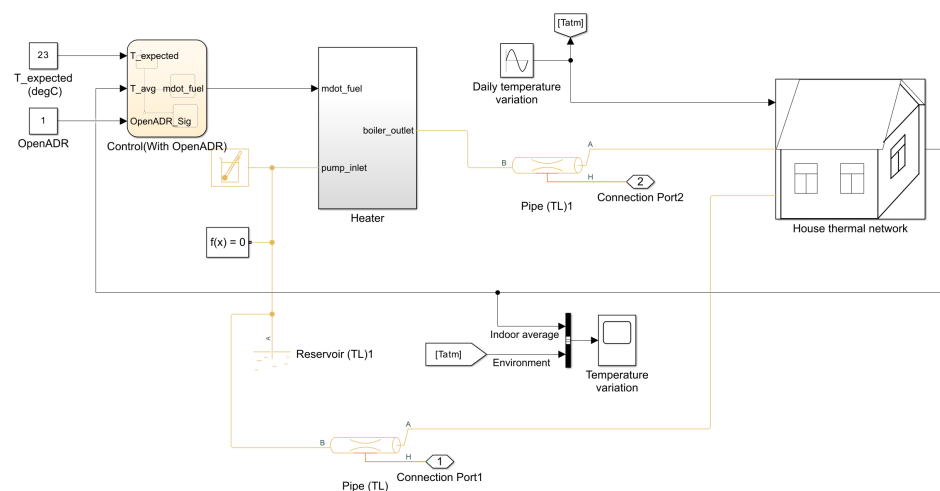
Figure 3. Layout of Scenario 2 on the simulation tool (with protocol).
