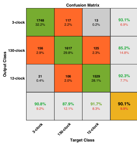
Fig. 4 Confusion matrix for the single-hand driving mode posture recognition with the MTS-Trans4 model
