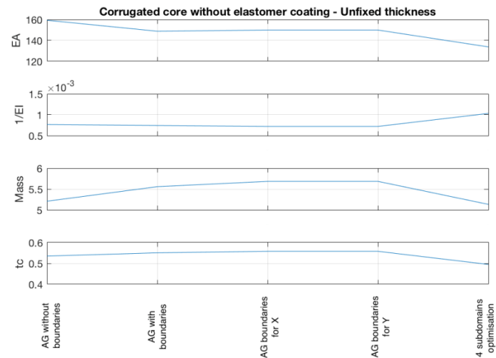
Figure 17 Comparative analysis of objective values and thickness of material for different optimisation approaches
