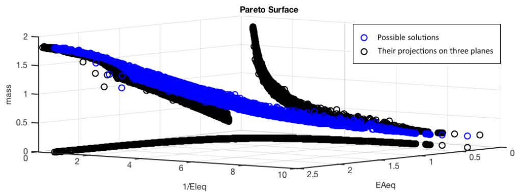
Figure 6 Pareto surface, multi-objective optimisation of corrugated skin (Aggregate optimisation method)
