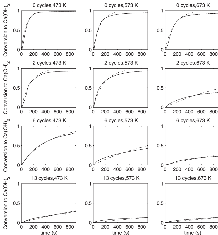
Fig. 4. Plots of projected conversion to \text{Ca(OH)}_2 as a function of time as calculated by the SCM (dashed lines) against experimental data (solid lines); note that all plots in the same y position have the same cycle number (0, 2, 6 or 13) and all in the same x position have the same hydration temperature (473, 573 or 673 K); x axis limits kept constant for experiments of the same cycle number.
