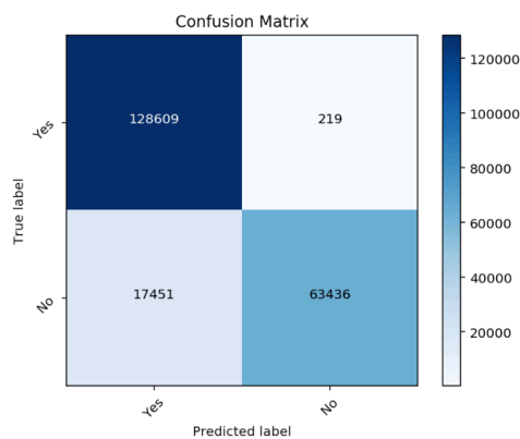
Figure 3: Confusion matrix of testing classification using DNN with an epoch=500
