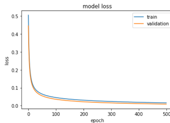
Figure 6: Model loss plot for DNN with epoch=500
