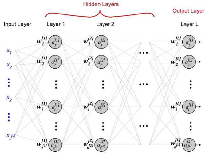
Figure 1: Architecture of Deep Feedforward Neural Network [43]
