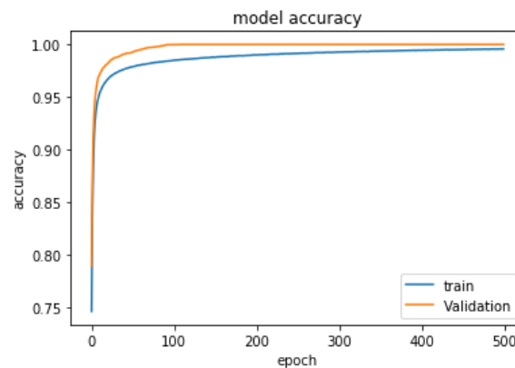
Figure 5: Model accuracy plot for DNN with epoch=500
