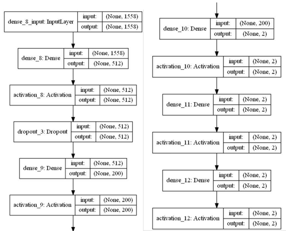
Figure 7: Final DNN Model architecture
