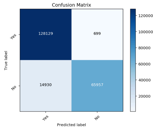
Figure 4: Confusion matrix of testing classification using DNN with an epoch=200
