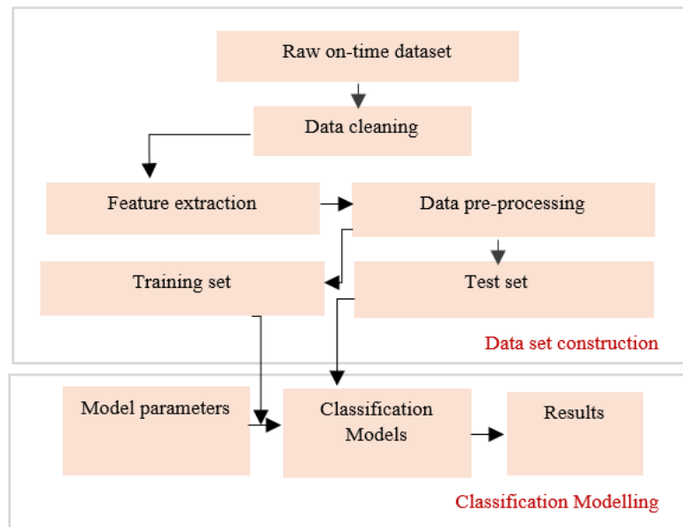
Figure 2: An overview of the experiment steps
