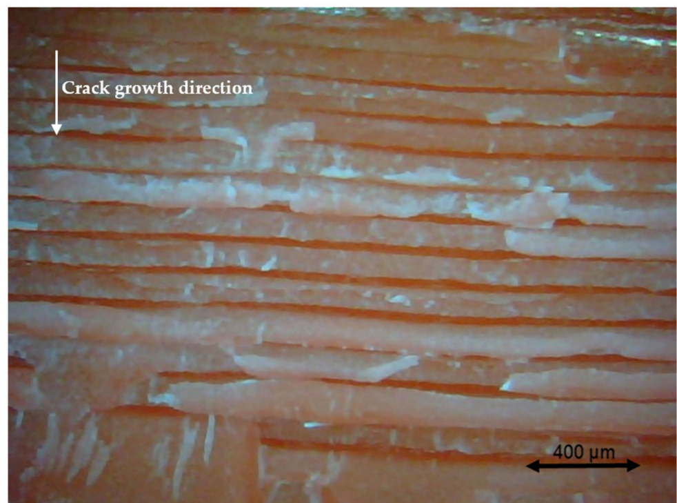
Figure 22. Specimen with a nozzle size of 0.6 mm, Y building orientation, and layer thickness of 0.1 mm.
