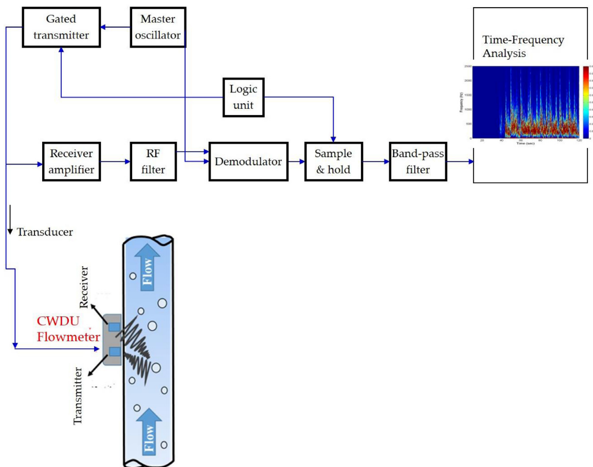
Fig. 2. Hardware block diagram of a continuous-wave Doppler ultrasound system (Nnabuiife, Sharma, et al., 2021)
