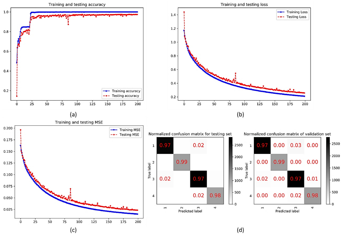
Fig. 17. The detailed experimental records of the CRNN1.0-based flow regime classifier using the augmentation scheme A (Experiment No.5)
