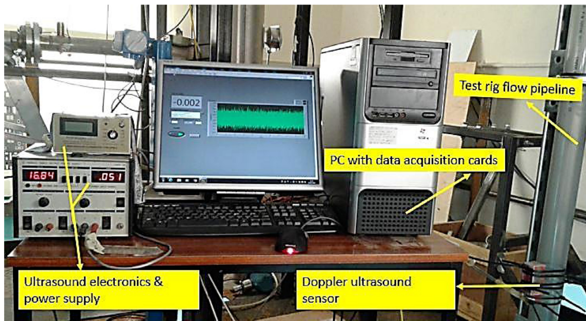
Fig. 3. The ultrasonic sensor and the auxiliary instruments used in this research (Nnabuiife et al., 2020).
