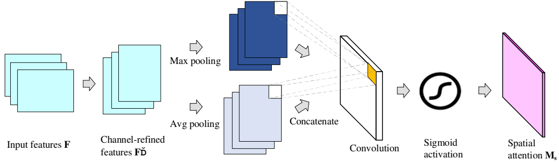
Figure 3. The flow chart of getting spatial attention
