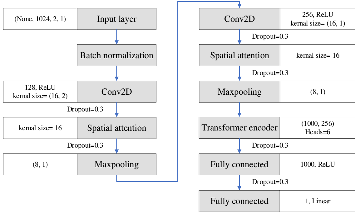
Figure 5. The parameters setting of SAConvFormer
