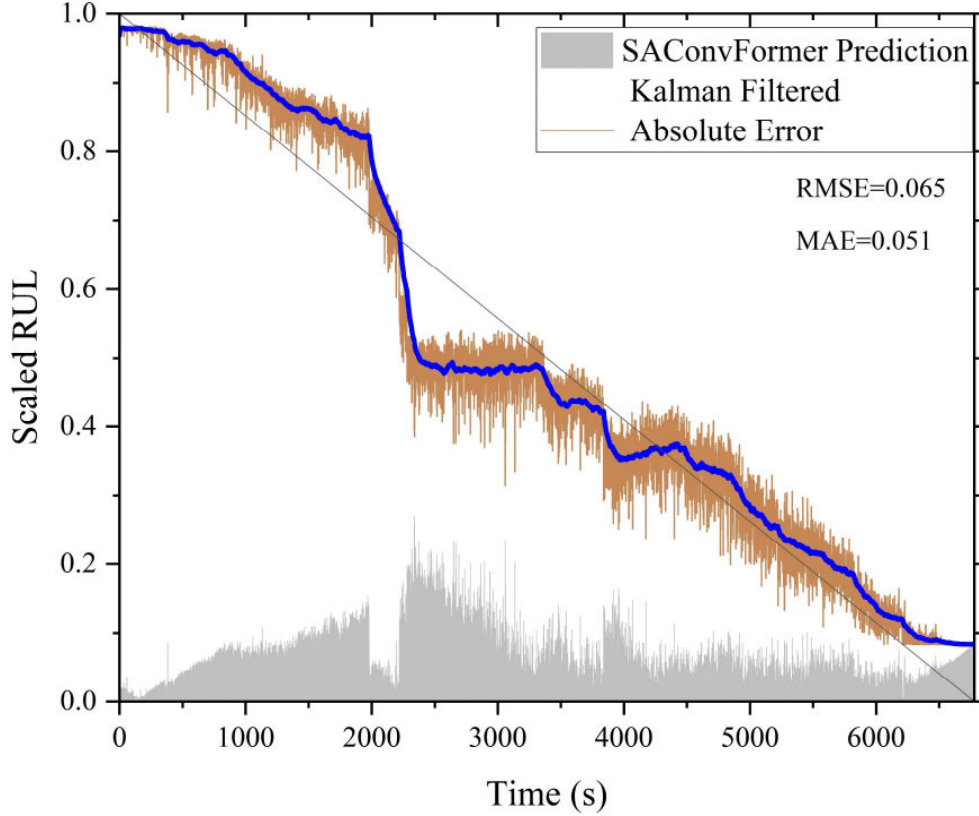
Figure 9. The prediction results for Bearing 2_2
