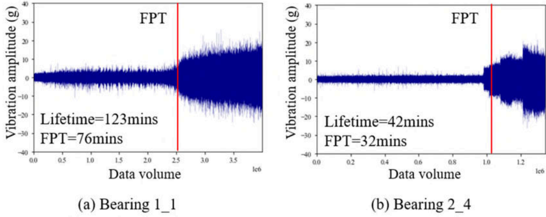
Figure 6. Demonstration of the horizontal vibration signals of (a) Bearing 1_1 and (b) Bearing 2_4
