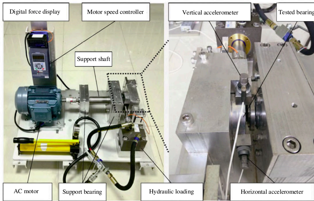
Figure 4. The tested platform of the rolling element bearing
