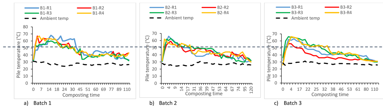
Fig. 3 Temperature profiles of batch piles (a, b, and c)
